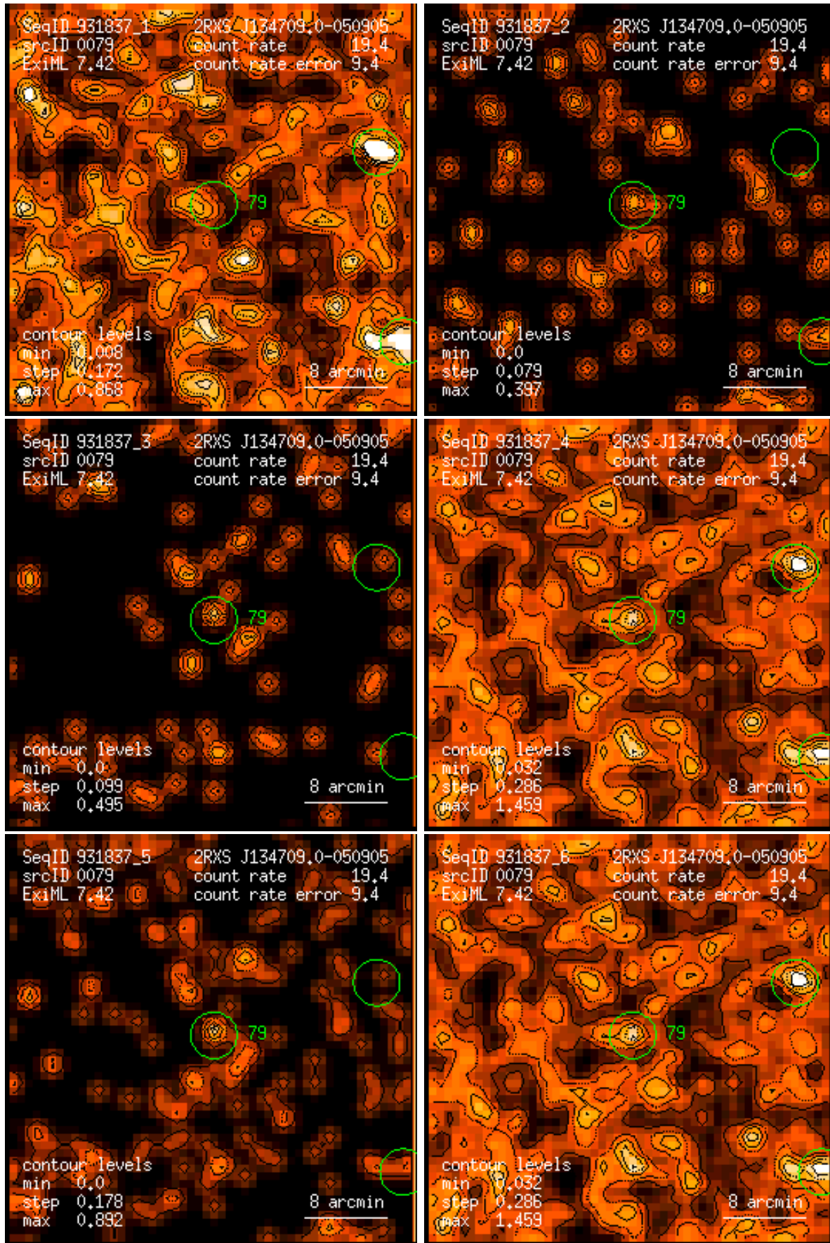
Figure 79: RASS 931837: detection 0079: band rate images, Gaussian filter: (1) PSPC channels 11 – 41, (2) 52 – 90, (3) 91 – 201, (4) 11 – 235, (5) 52 – 201, (6) 11 – 201. Broad band rates in counts/ks. Band rate contour levels in counts/ks/arcmin 2 .
