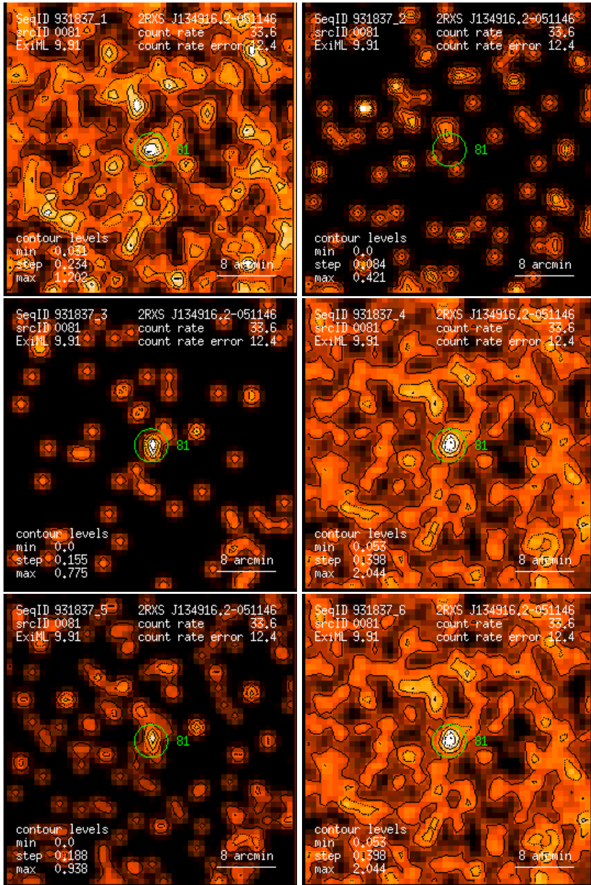
Figure 81: RASS 931837: detection 0081: band rate images, Gaussian filter: (1) PSPC channels 11 – 41, (2) 52 – 90, (3) 91 – 201, (4) 11 – 235, (5) 52 – 201, (6) 11 – 201. Broad band rates in counts/ks. Band rate contour levels in counts/ks/arcmin 2 .
