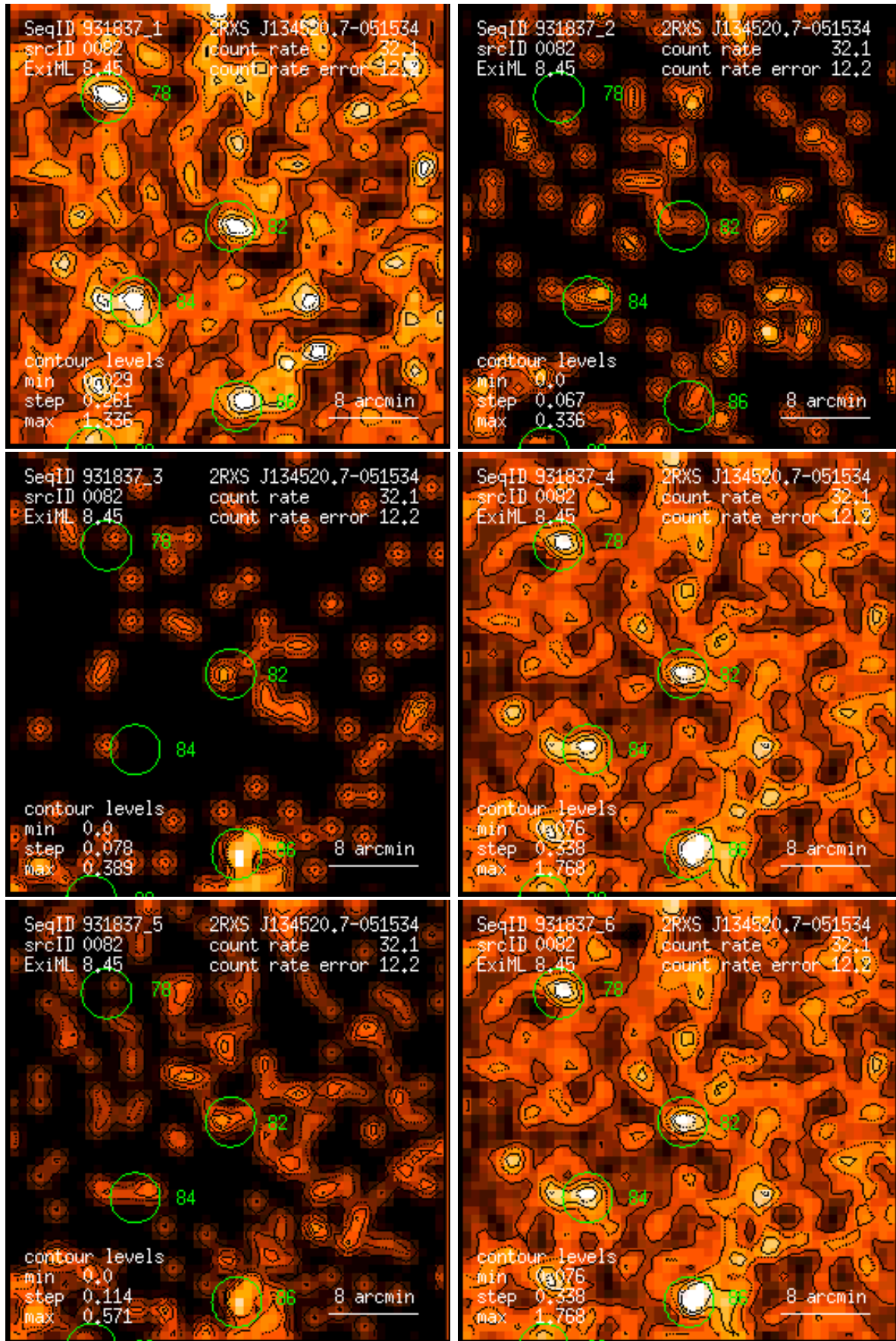
Figure 82: RASS 931837: detection 0082: band rate images, Gaussian filter: (1) PSPC channels 11 – 41, (2) 52 – 90, (3) 91 – 201, (4) 11 – 235, (5) 52 – 201, (6) 11 – 201. Broad band rates in counts/ks. Band rate contour levels in counts/ks/arcmin 2 .
