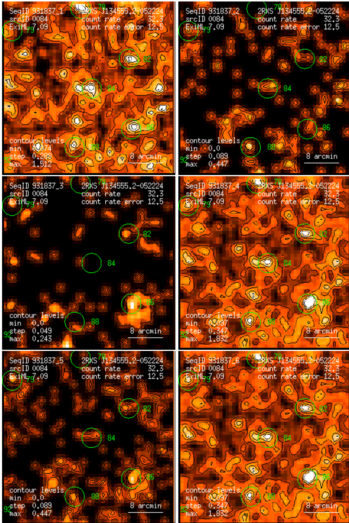
Figure 84: RASS 931837: detection 0084: band rate images, Gaussian filter: (1) PSPC channels 11 – 41, (2) 52 – 90, (3) 91 – 201, (4) 11 – 235, (5) 52 – 201, (6) 11 – 201. Broad band rates in counts/ks. Band rate contour levels in counts/ks/arcmin 2 .
