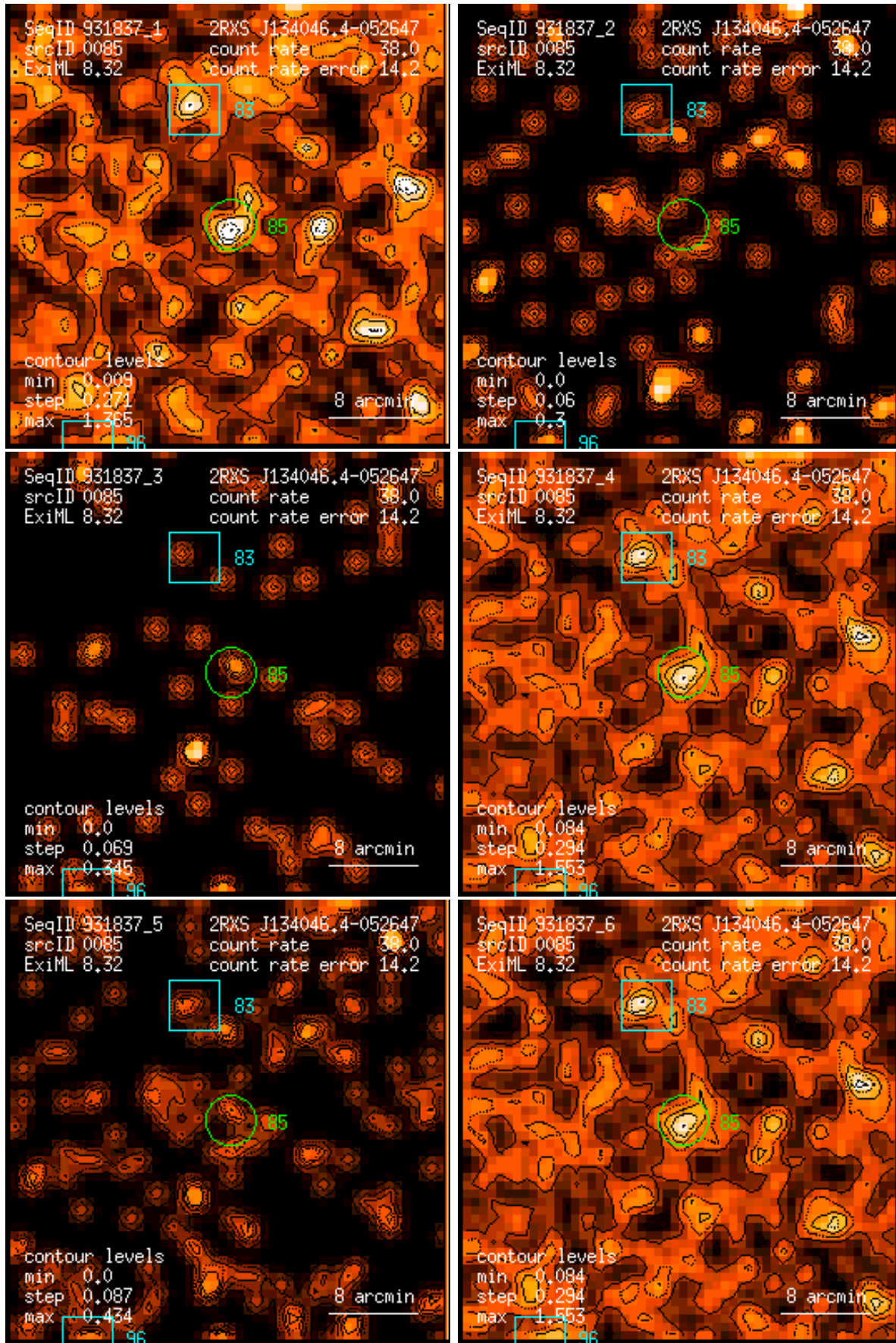
Figure 85: RASS 931837: detection 0085: band rate images, Gaussian filter: (1) PSPC channels 11 – 41, (2) 52 – 90, (3) 91 – 201, (4) 11 – 235, (5) 52 – 201, (6) 11 – 201. Broad band rates in counts/ks. Band rate contour levels in counts/ks/arcmin 2 .
