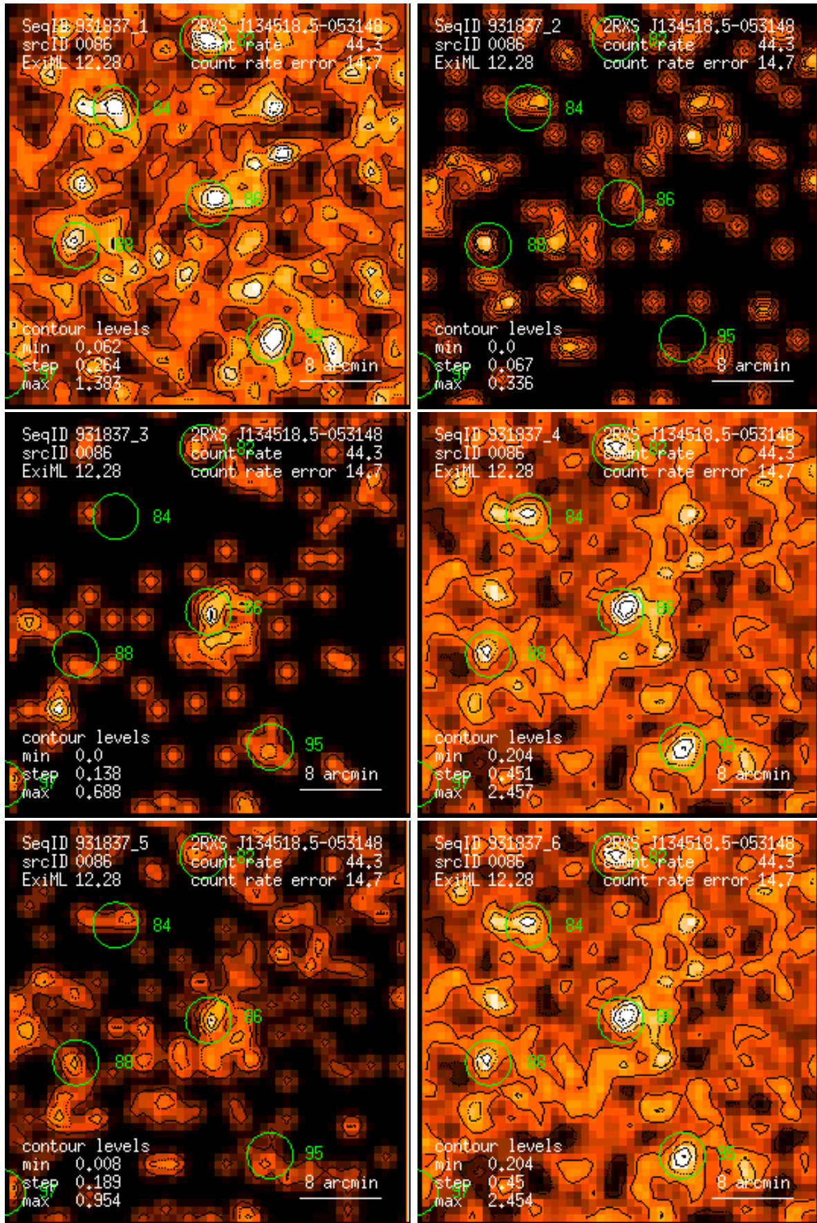
Figure 86: RASS 931837: detection 0086: band rate images, Gaussian filter: (1) PSPC channels 11 – 41, (2) 52 – 90, (3) 91 – 201, (4) 11 – 235, (5) 52 – 201, (6) 11 – 201. Broad band rates in counts/ks. Band rate contour levels in counts/ks/arcmin 2 .
