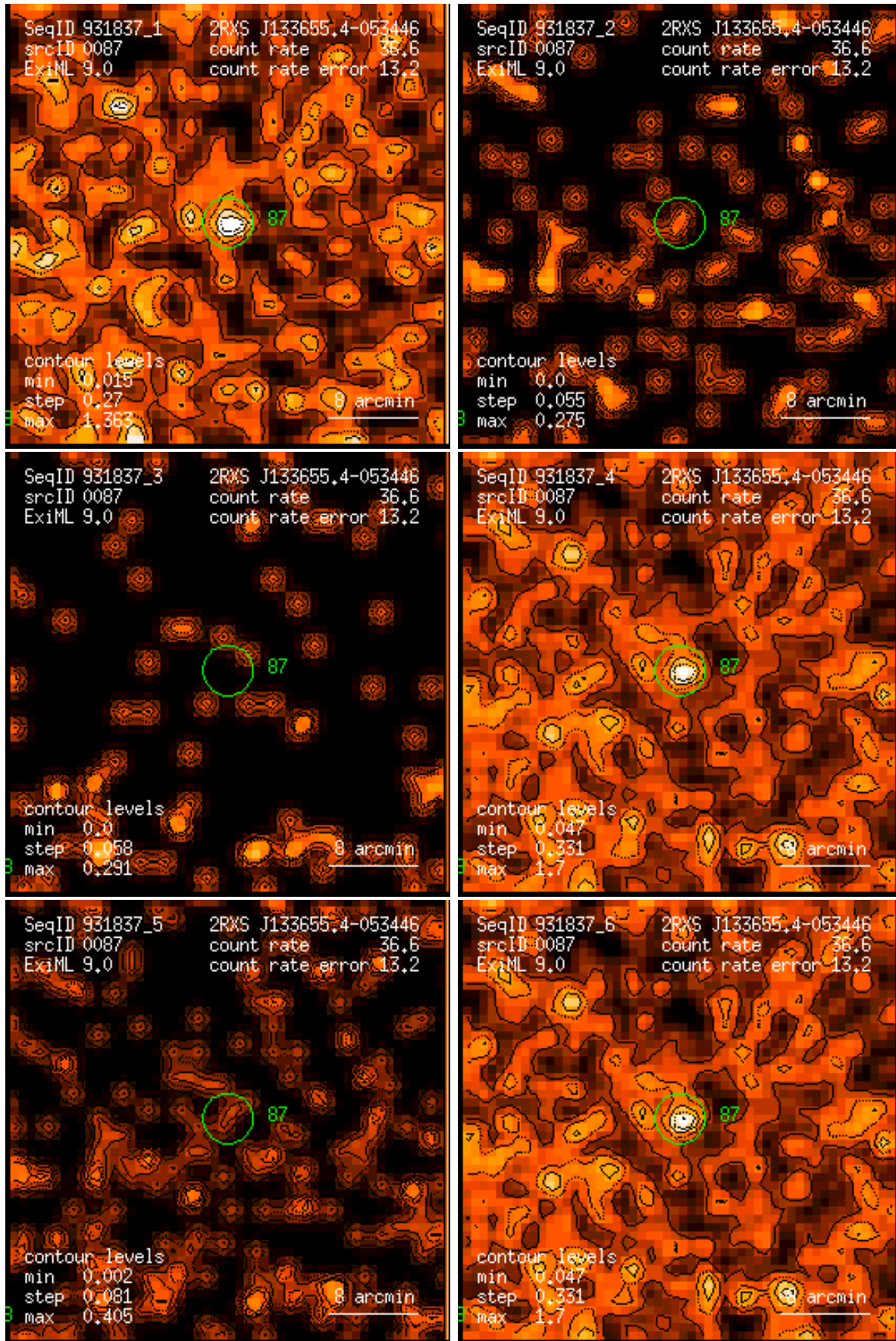
Figure 87: RASS 931837: detection 0087: band rate images, Gaussian filter: (1) PSPC channels 11 – 41, (2) 52 – 90, (3) 91 – 201, (4) 11 – 235, (5) 52 – 201, (6) 11 – 201. Broad band rates in counts/ks. Band rate contour levels in counts/ks/arcmin 2 .
