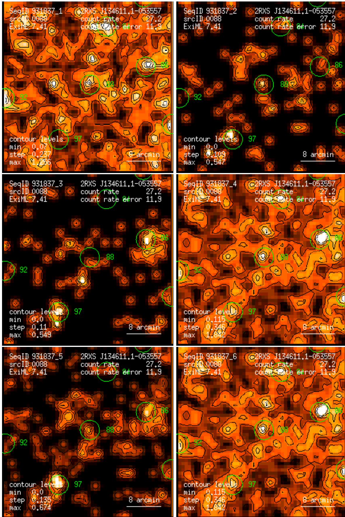
Figure 88: RASS 931837: detection 0088: band rate images, Gaussian filter: (1) PSPC channels 11 – 41, (2) 52 – 90, (3) 91 – 201, (4) 11 – 235, (5) 52 – 201, (6) 11 – 201. Broad band rates in counts/ks. Band rate contour levels in counts/ks/arcmin 2 .
