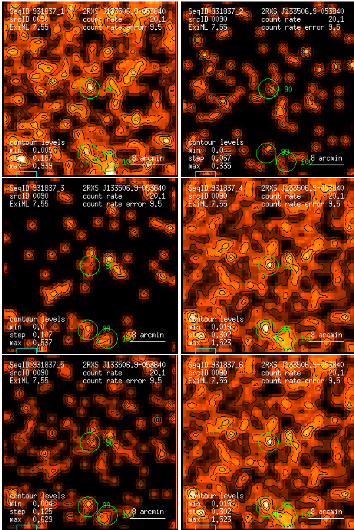
Figure 90: RASS 931837: detection 0090: band rate images, Gaussian filter: (1) PSPC channels 11 – 41, (2) 52 – 90, (3) 91 – 201, (4) 11 – 235, (5) 52 – 201, (6) 11 – 201. Broad band rates in counts/ks. Band rate contour levels in counts/ks/arcmin 2 .
