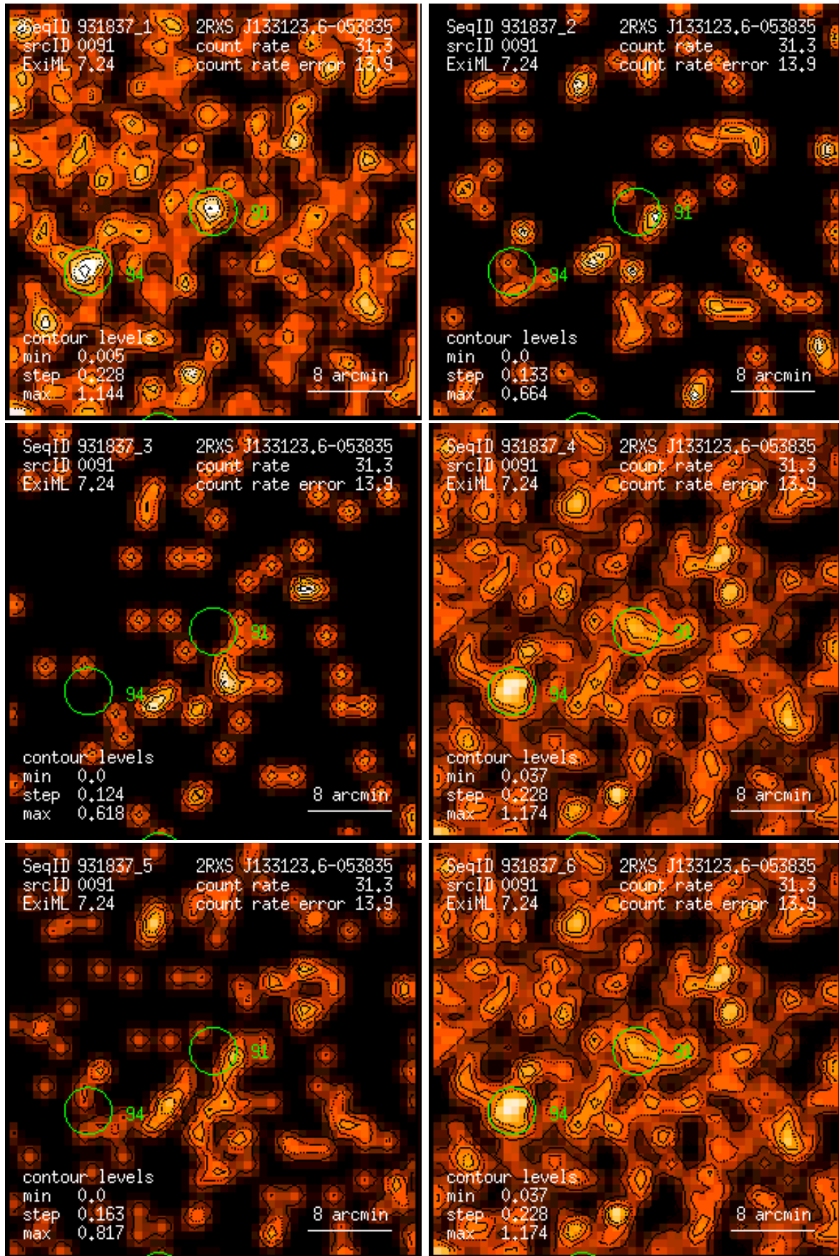
Figure 91: RASS 931837: detection 0091: band rate images, Gaussian filter: (1) PSPC channels 11 – 41, (2) 52 – 90, (3) 91 – 201, (4) 11 – 235, (5) 52 – 201, (6) 11 – 201. Broad band rates in counts/ks. Band rate contour levels in counts/ks/arcmin 2 .
