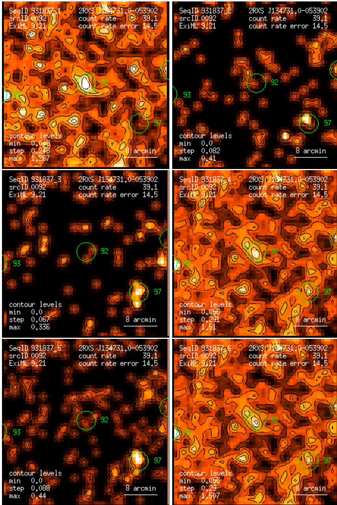
Figure 92: RASS 931837: detection 0092: band rate images, Gaussian filter: (1) PSPC channels 11 – 41, (2) 52 – 90, (3) 91 – 201, (4) 11 – 235, (5) 52 – 201, (6) 11 – 201. Broad band rates in counts/ks. Band rate contour levels in counts/ks/arcmin 2 .
