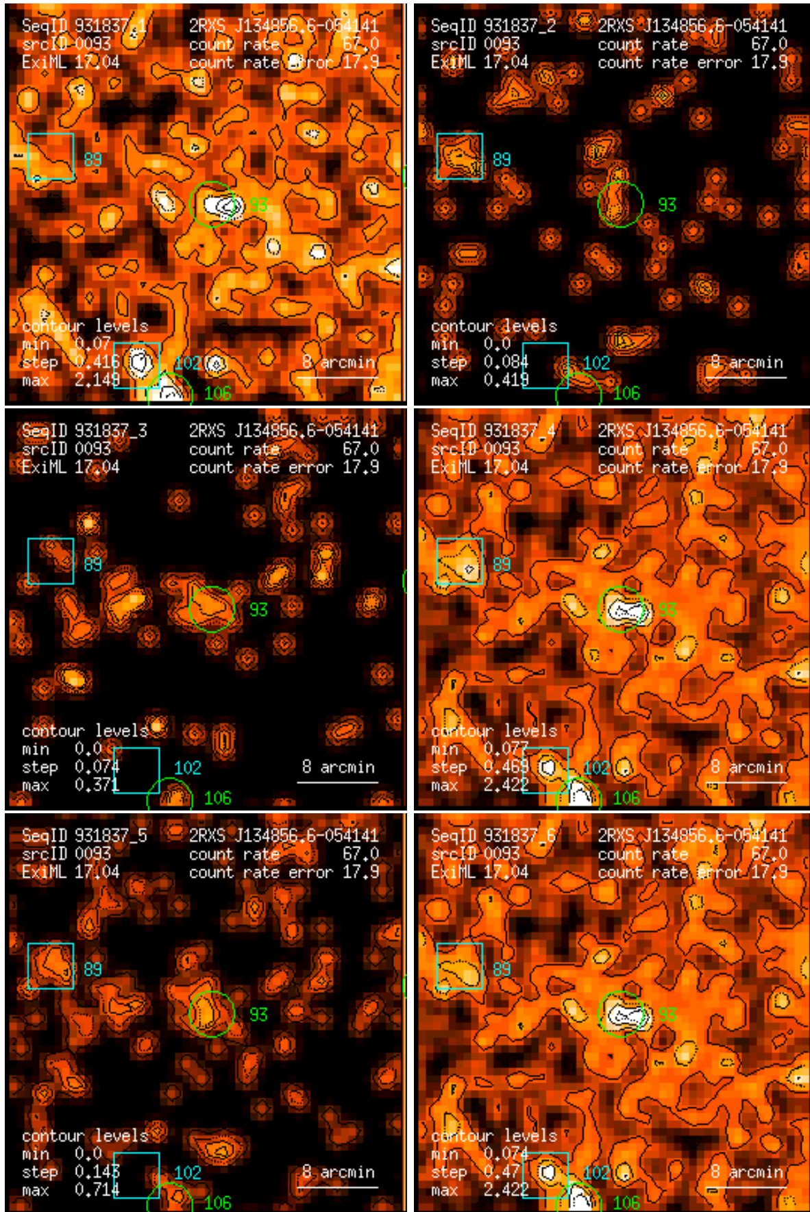
Figure 93: RASS 931837: detection 0093: band rate images, Gaussian filter: (1) PSPC channels 11 – 41, (2) 52 – 90, (3) 91 – 201, (4) 11 – 235, (5) 52 – 201, (6) 11 – 201. Broad band rates in counts/ks. Band rate contour levels in counts/ks/arcmin 2 .
