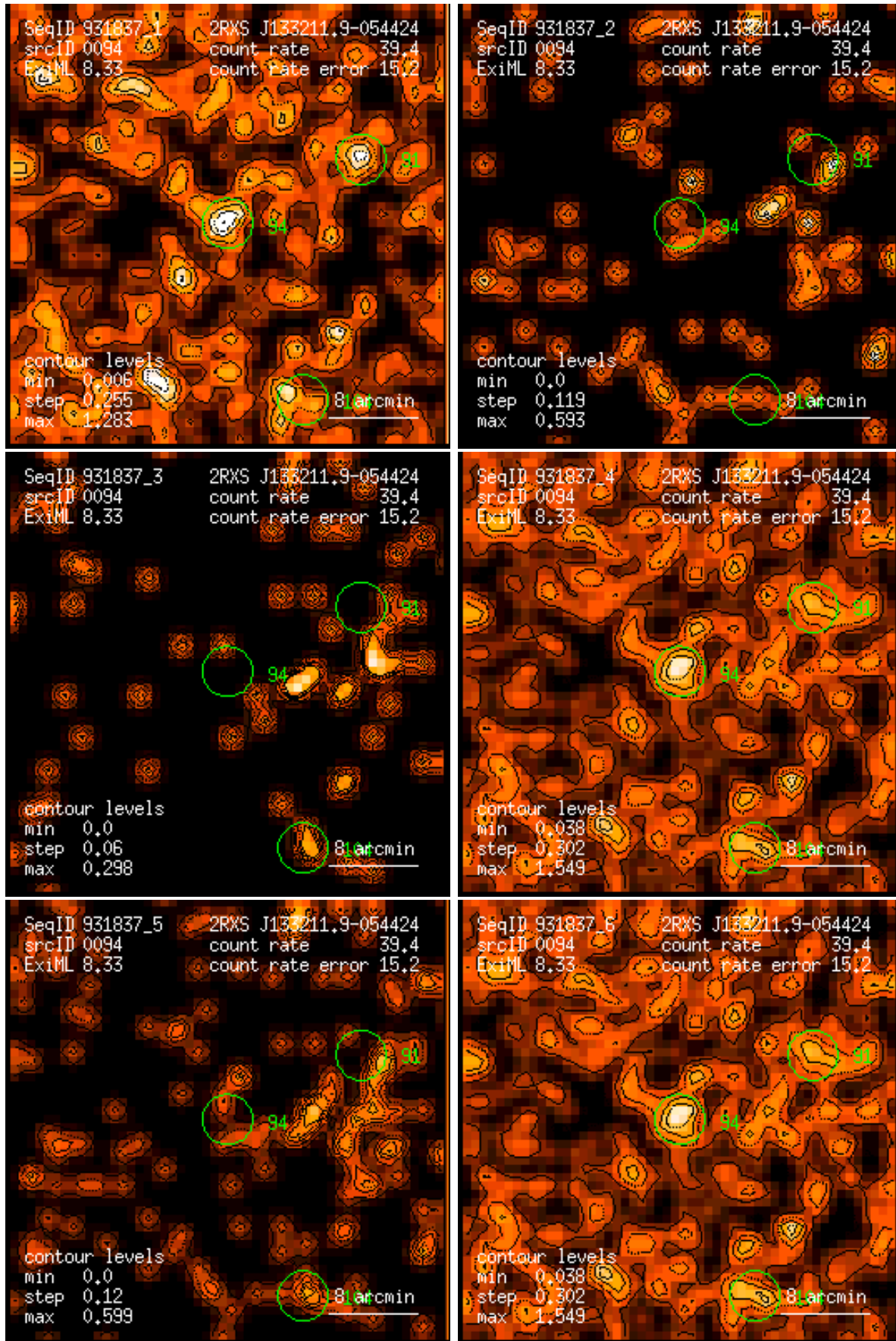
Figure 94: RASS 931837: detection 0094: band rate images, Gaussian filter: (1) PSPC channels 11 – 41, (2) 52 – 90, (3) 91 – 201, (4) 11 – 235, (5) 52 – 201, (6) 11 – 201. Broad band rates in counts/ks. Band rate contour levels in counts/ks/arcmin 2 .
