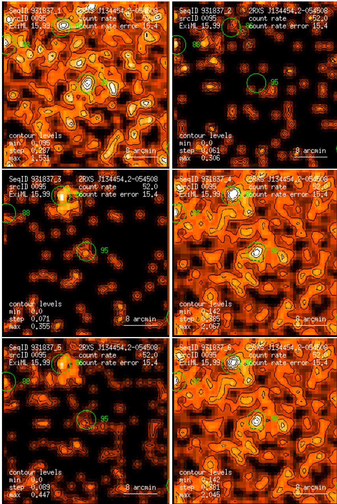
Figure 95: RASS 931837: detection 0095: band rate images, Gaussian filter: (1) PSPC channels 11 – 41, (2) 52 – 90, (3) 91 – 201, (4) 11 – 235, (5) 52 – 201, (6) 11 – 201. Broad band rates in counts/ks. Band rate contour levels in counts/ks/arcmin 2 .
