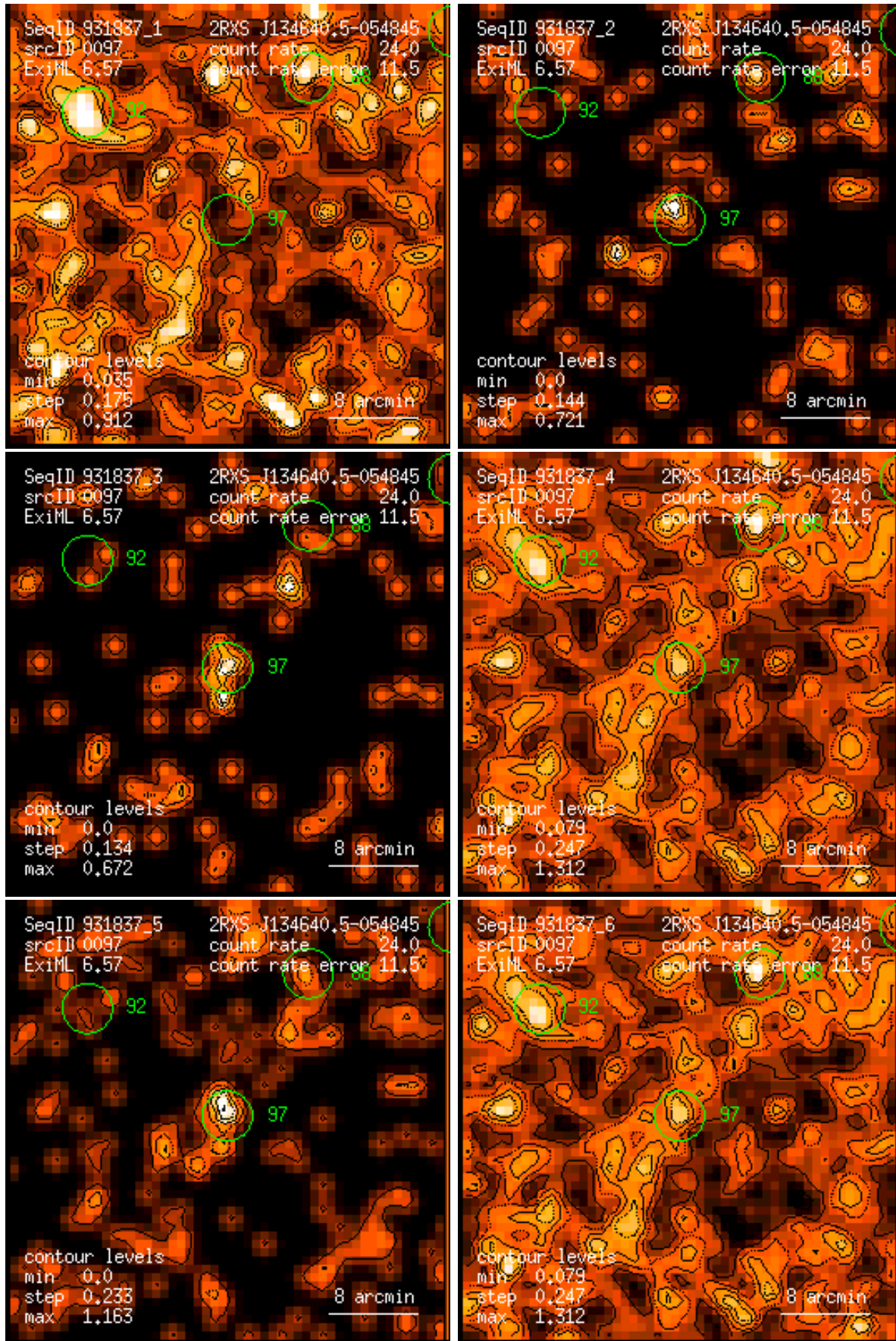
Figure 97: RASS 931837: detection 0097: band rate images, Gaussian filter: (1) PSPC channels 11 – 41, (2) 52 – 90, (3) 91 – 201, (4) 11 – 235, (5) 52 – 201, (6) 11 – 201. Broad band rates in counts/ks. Band rate contour levels in counts/ks/arcmin 2 .
