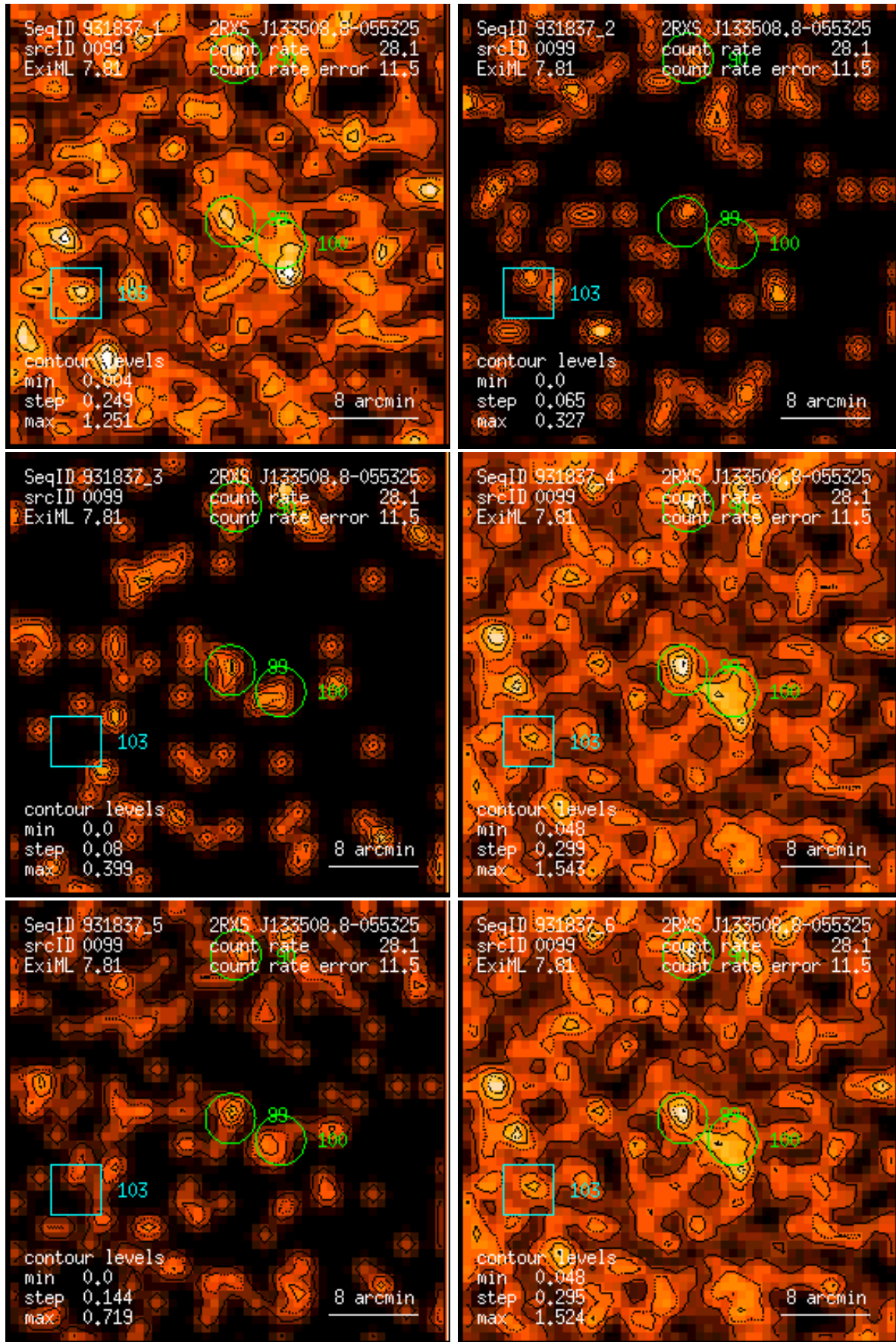
Figure 99: RASS 931837: detection 0099: band rate images, Gaussian filter: (1) PSPC channels 11 – 41, (2) 52 – 90, (3) 91 – 201, (4) 11 – 235, (5) 52 – 201, (6) 11 – 201. Broad band rates in counts/ks. Band rate contour levels in counts/ks/arcmin 2 .
