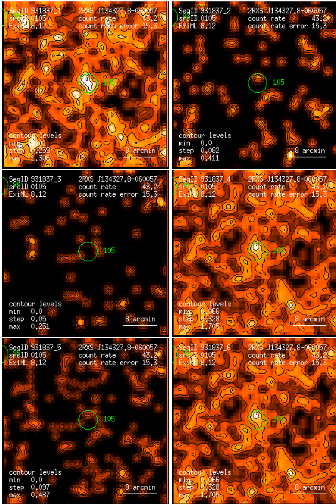
Figure 105: RASS 931837: detection 0105: band rate images, Gaussian filter: (1) PSPC channels 11 – 41, (2) 52 – 90, (3) 91 – 201, (4) 11 – 235, (5) 52 – 201, (6) 11 – 201. Broad band rates in counts/ks. Band rate contour levels in counts/ks/arcmin 2 .
