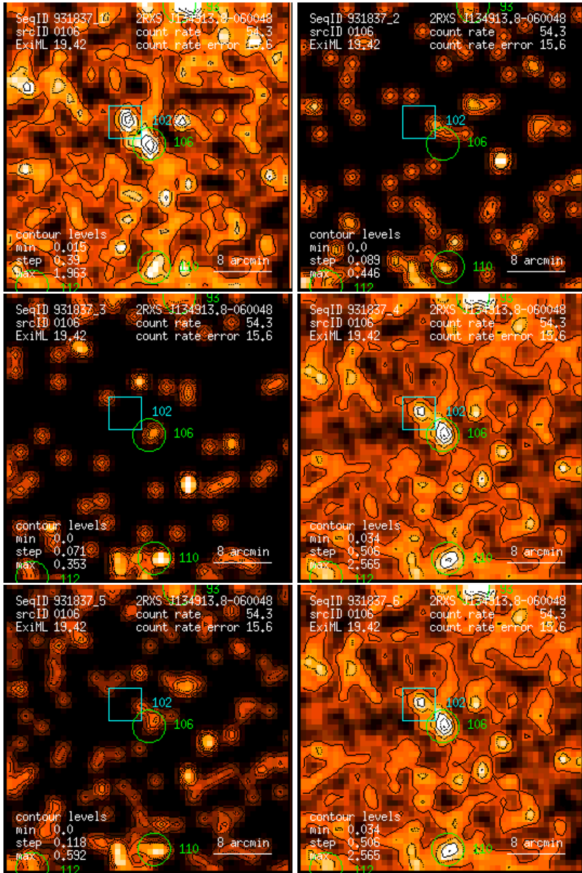
Figure 106: RASS 931837: detection 0106: band rate images, Gaussian filter: (1) PSPC channels 11 – 41, (2) 52 – 90, (3) 91 – 201, (4) 11 – 235, (5) 52 – 201, (6) 11 – 201. Broad band rates in counts/ks. Band rate contour levels in counts/ks/arcmin 2 .
