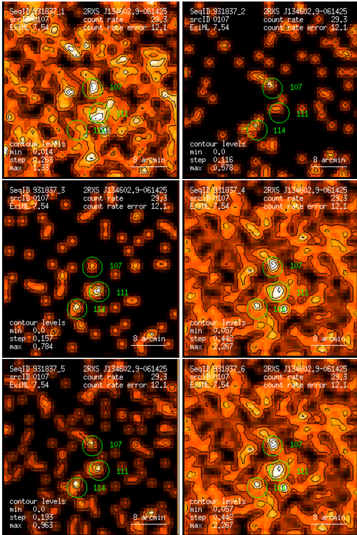
Figure 107: RASS 931837: detection 0107: band rate images, Gaussian filter: (1) PSPC channels 11 – 41, (2) 52 – 90, (3) 91 – 201, (4) 11 – 235, (5) 52 – 201, (6) 11 – 201. Broad band rates in counts/ks. Band rate contour levels in counts/ks/arcmin 2 .
