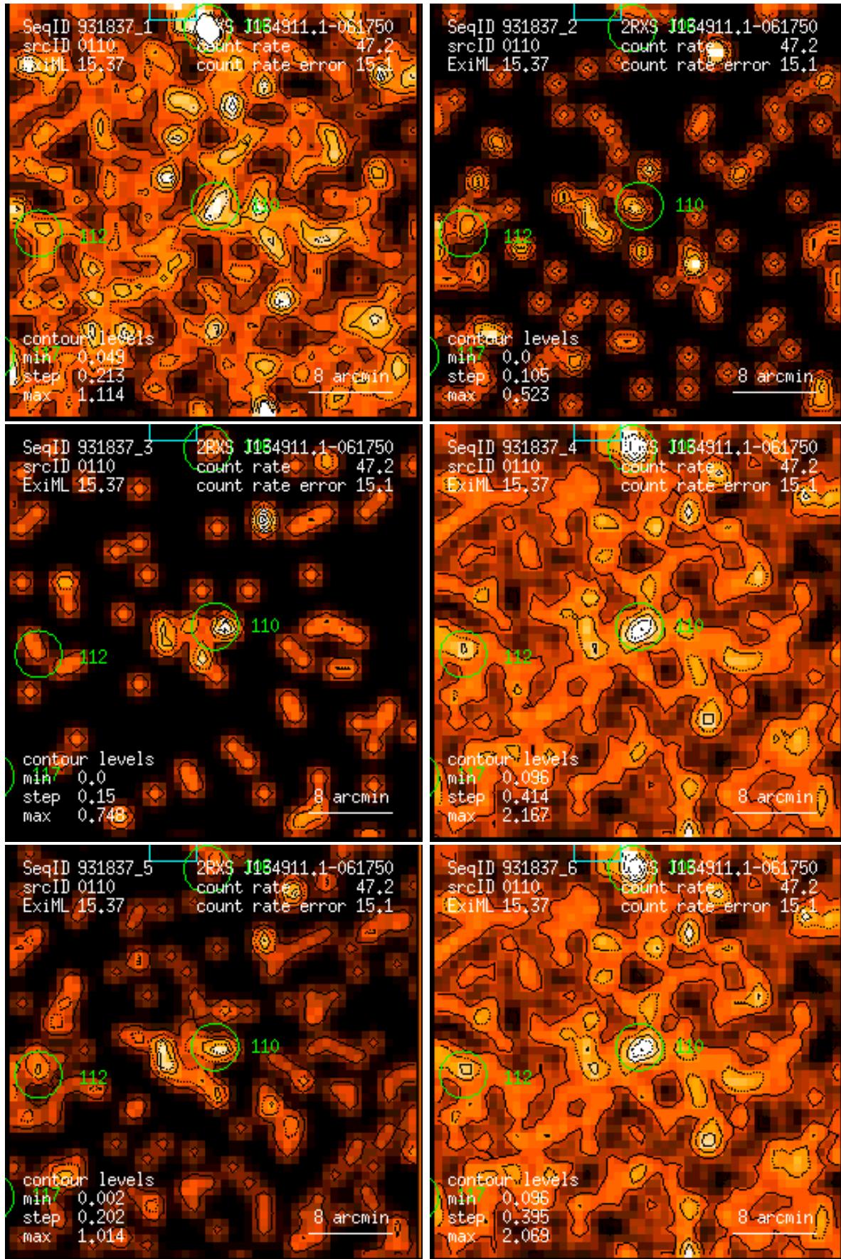
Figure 110: RASS 931837: detection 0110: band rate images, Gaussian filter: (1) PSPC channels 11 – 41, (2) 52 – 90, (3) 91 – 201, (4) 11 – 235, (5) 52 – 201, (6) 11 – 201. Broad band rates in counts/ks. Band rate contour levels in counts/ks/arcmin 2 .
