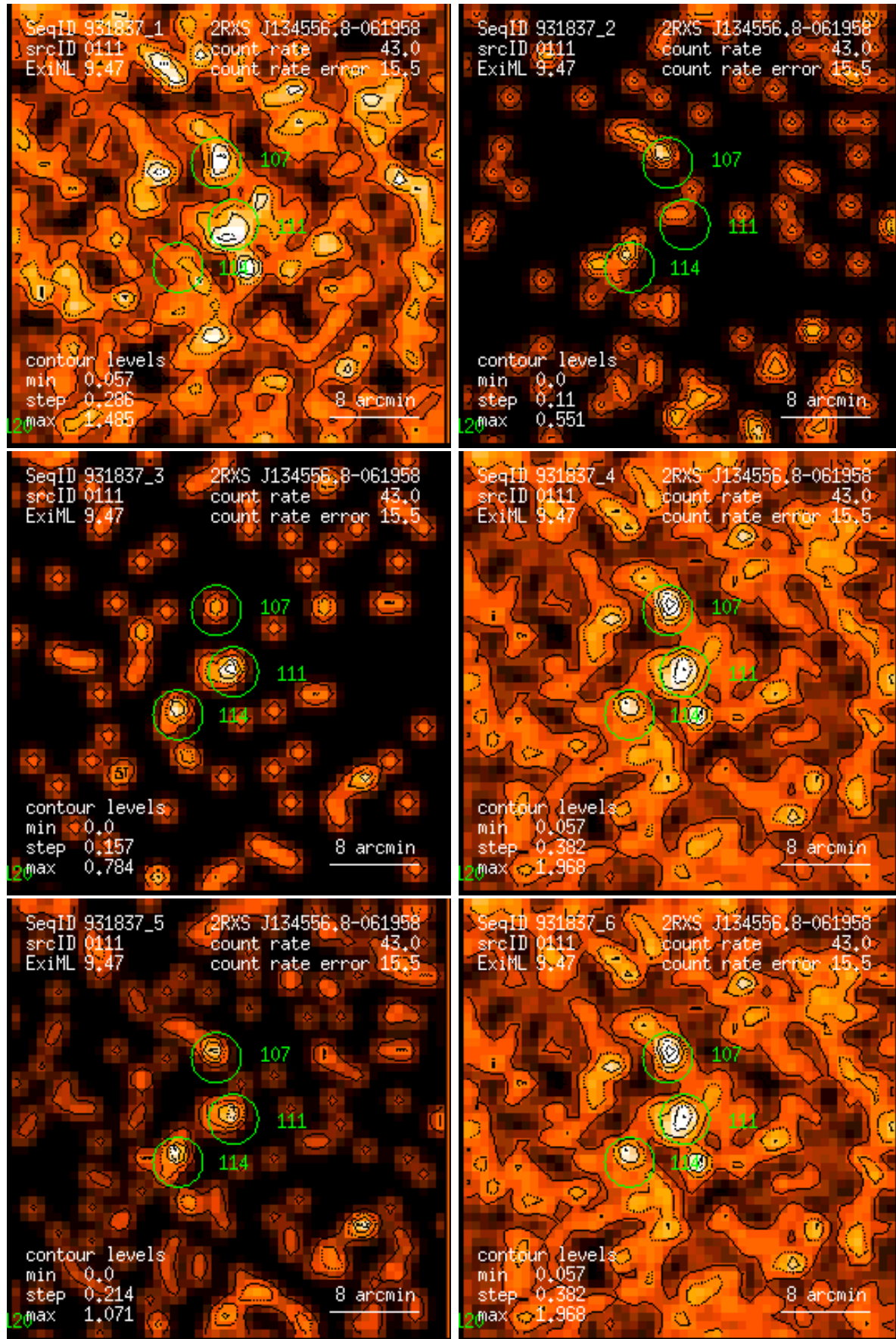
Figure 111: RASS 931837: detection 0111: band rate images, Gaussian filter: (1) PSPC channels 11 – 41, (2) 52 – 90, (3) 91 – 201, (4) 11 – 235, (5) 52 – 201, (6) 11 – 201. Broad band rates in counts/ks. Band rate contour levels in counts/ks/arcmin 2 .
