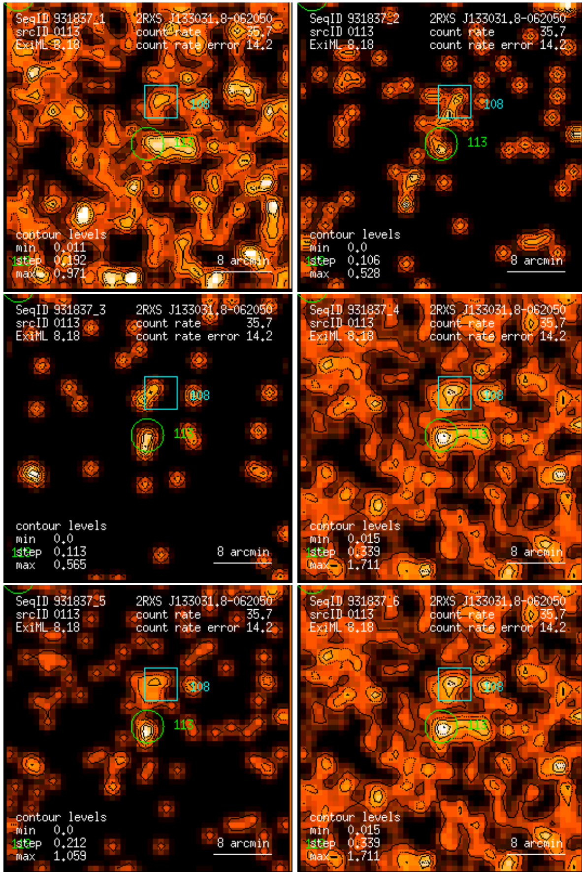
Figure 113: RASS 931837: detection 0113: band rate images, Gaussian filter: (1) PSPC channels 11 – 41, (2) 52 – 90, (3) 91 – 201, (4) 11 – 235, (5) 52 – 201, (6) 11 – 201. Broad band rates in counts/ks. Band rate contour levels in counts/ks/arcmin 2 .
