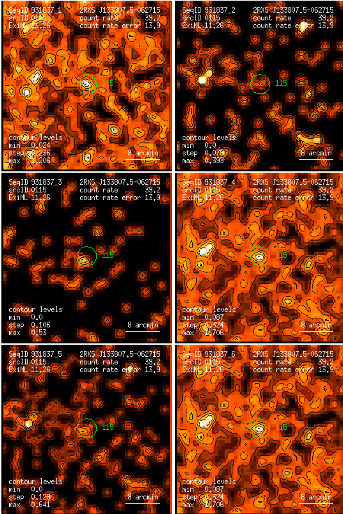
Figure 115: RASS 931837: detection 0115: band rate images, Gaussian filter: (1) PSPC channels 11 – 41, (2) 52 – 90, (3) 91 – 201, (4) 11 – 235, (5) 52 – 201, (6) 11 – 201. Broad band rates in counts/ks. Band rate contour levels in counts/ks/arcmin 2 .
