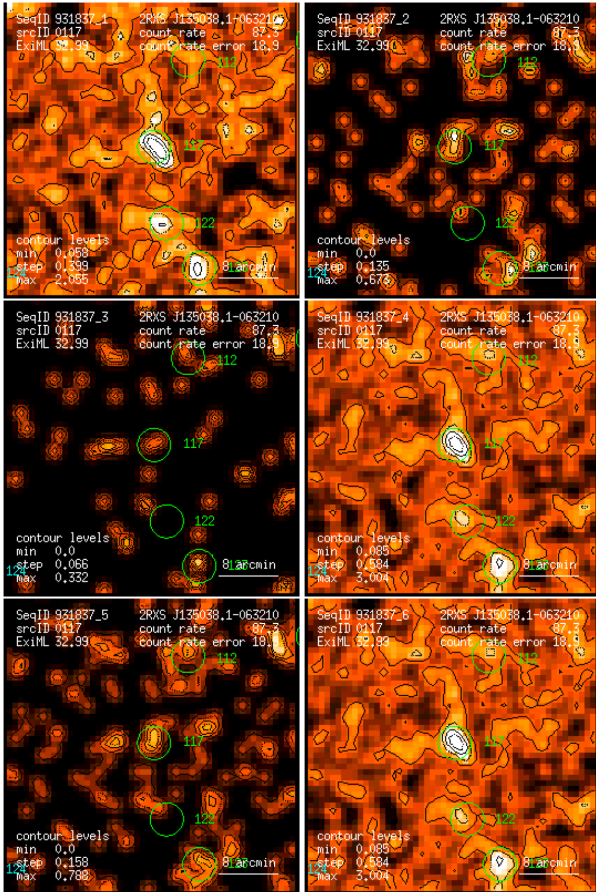
Figure 117: RASS 931837: detection 0117: band rate images, Gaussian filter: (1) PSPC channels 11 – 41, (2) 52 – 90, (3) 91 – 201, (4) 11 – 235, (5) 52 – 201, (6) 11 – 201. Broad band rates in counts/ks. Band rate contour levels in counts/ks/arcmin 2 .
