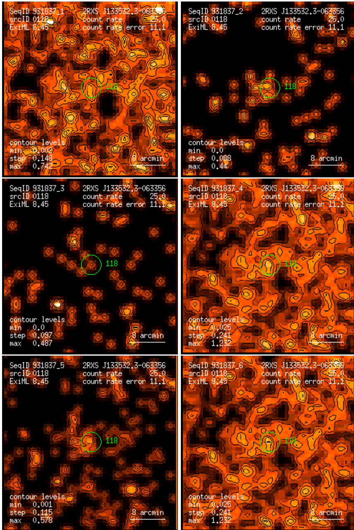
Figure 118: RASS 931837: detection 0118: band rate images, Gaussian filter: (1) PSPC channels 11 – 41, (2) 52 – 90, (3) 91 – 201, (4) 11 – 235, (5) 52 – 201, (6) 11 – 201. Broad band rates in counts/ks. Band rate contour levels in counts/ks/arcmin 2 .
