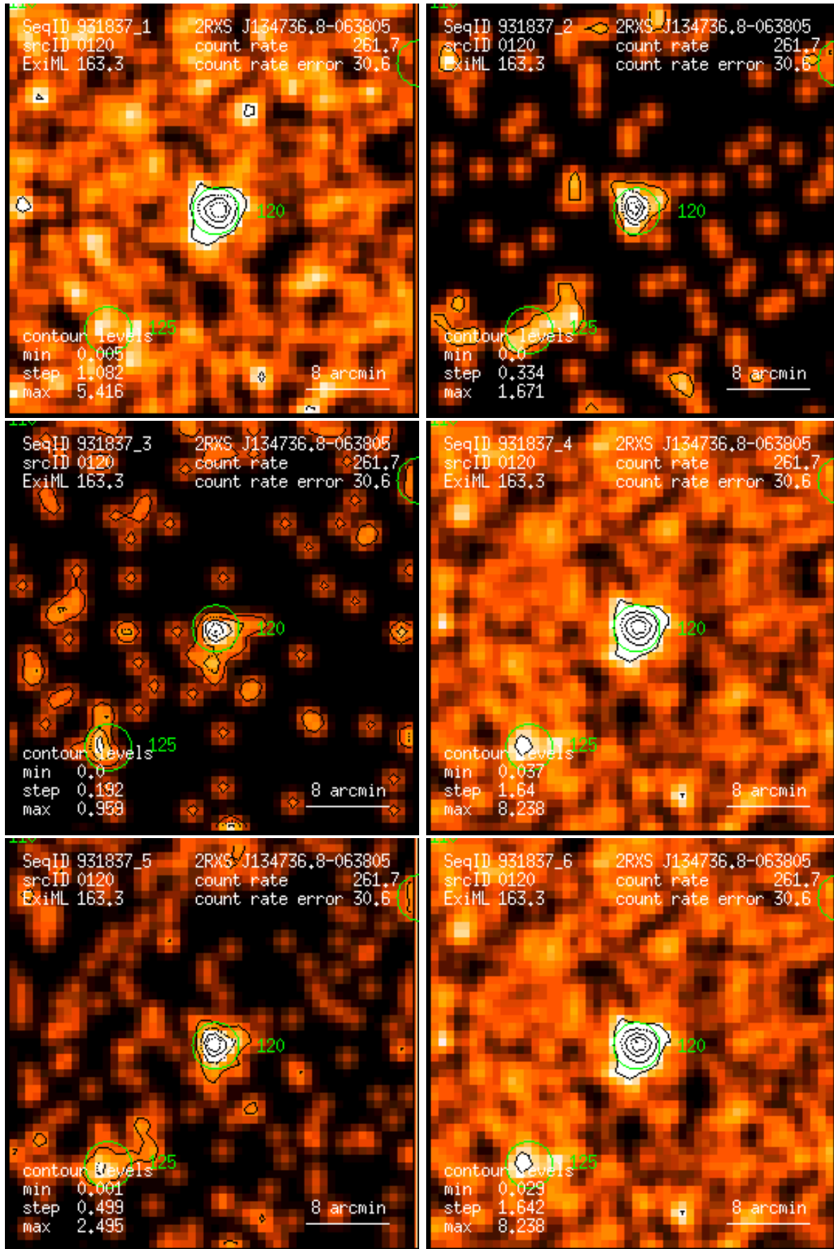
Figure 120: RASS 931837: detection 0120: band rate images, Gaussian filter: (1) PSPC channels 11 – 41, (2) 52 – 90, (3) 91 – 201, (4) 11 – 235, (5) 52 – 201, (6) 11 – 201. Broad band rates in counts/ks. Band rate contour levels in counts/ks/arcmin 2 .
