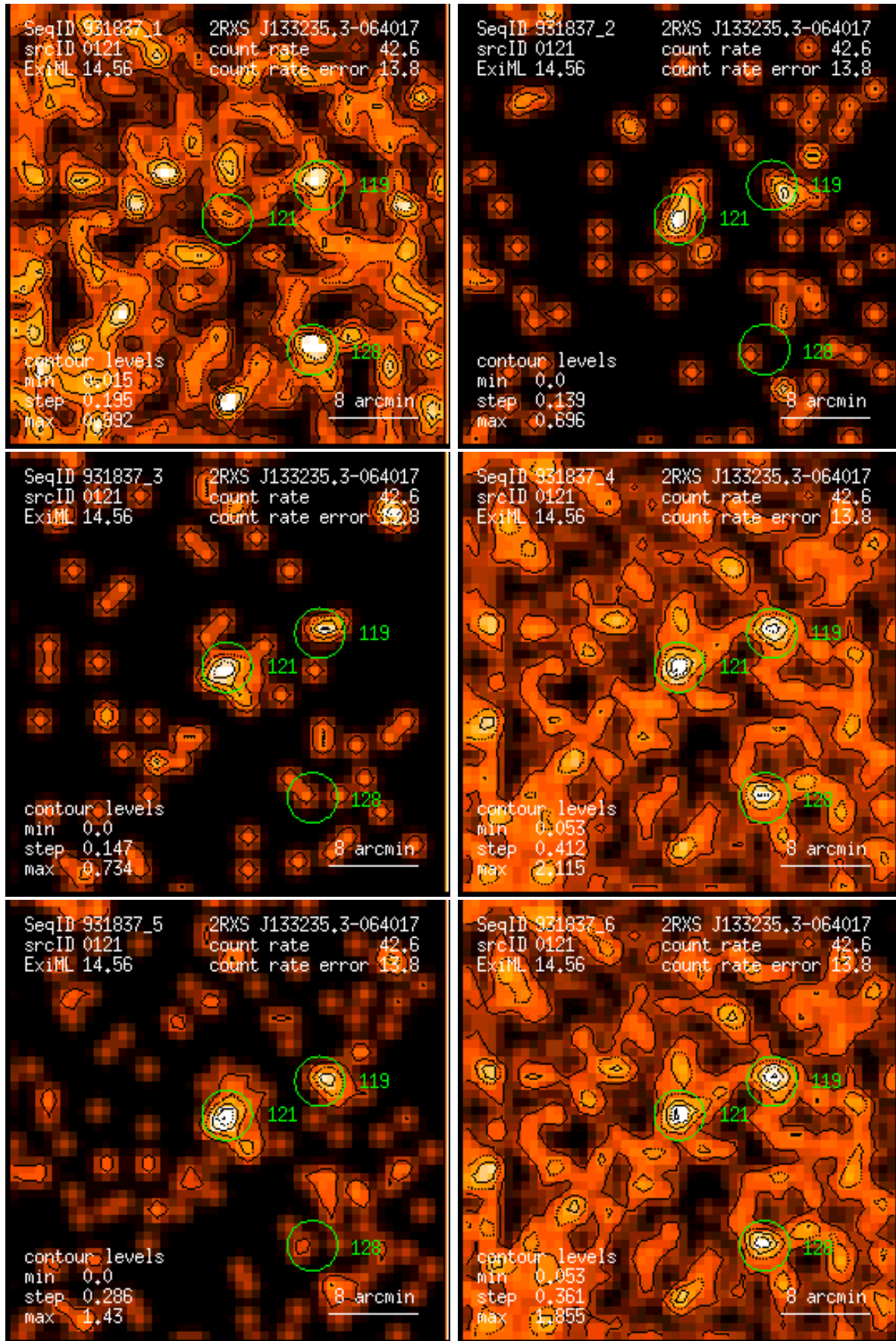
Figure 121: RASS 931837: detection 0121: band rate images, Gaussian filter: (1) PSPC channels 11 – 41, (2) 52 – 90, (3) 91 – 201, (4) 11 – 235, (5) 52 – 201, (6) 11 – 201. Broad band rates in counts/ks. Band rate contour levels in counts/ks/arcmin 2 .
