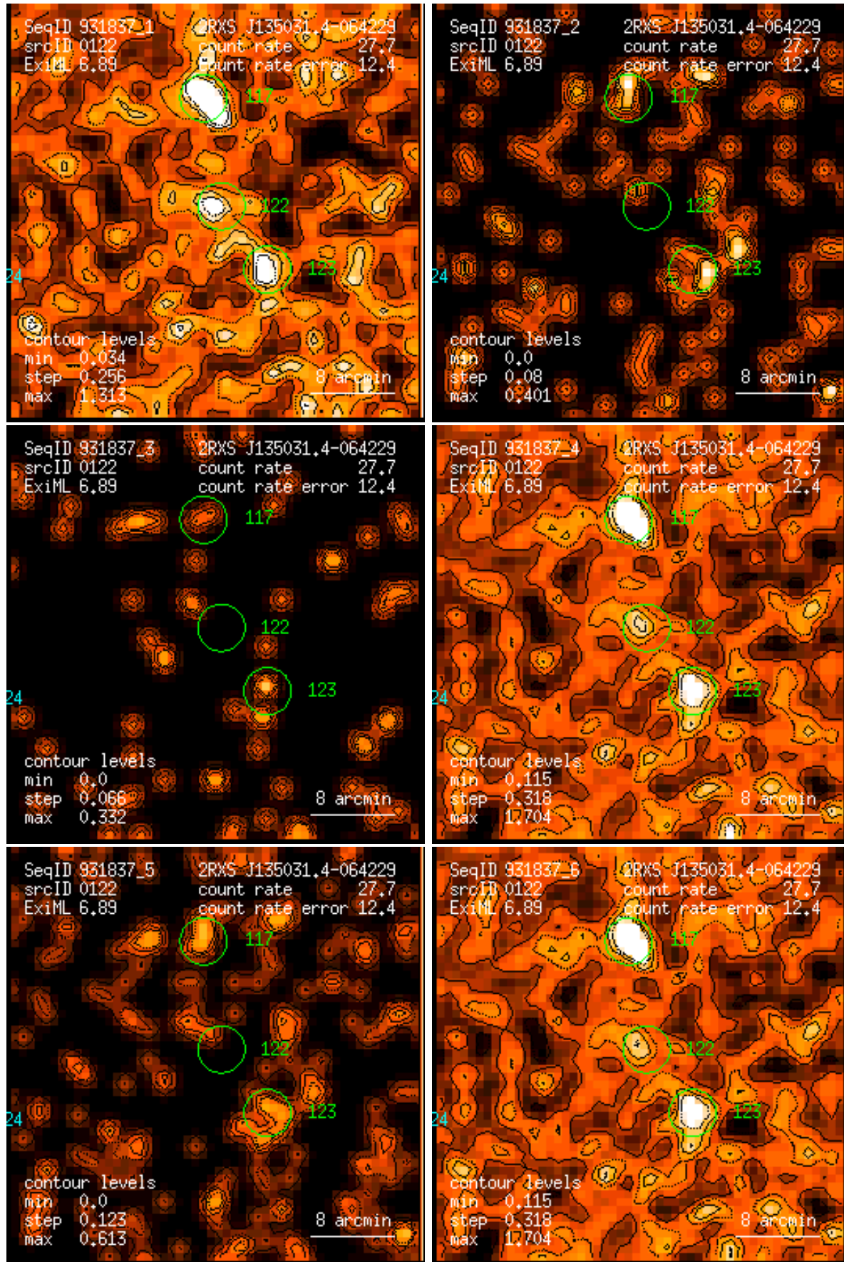
Figure 122: RASS 931837: detection 0122: band rate images, Gaussian filter: (1) PSPC channels 11 – 41, (2) 52 – 90, (3) 91 – 201, (4) 11 – 235, (5) 52 – 201, (6) 11 – 201. Broad band rates in counts/ks. Band rate contour levels in counts/ks/arcmin 2 .
