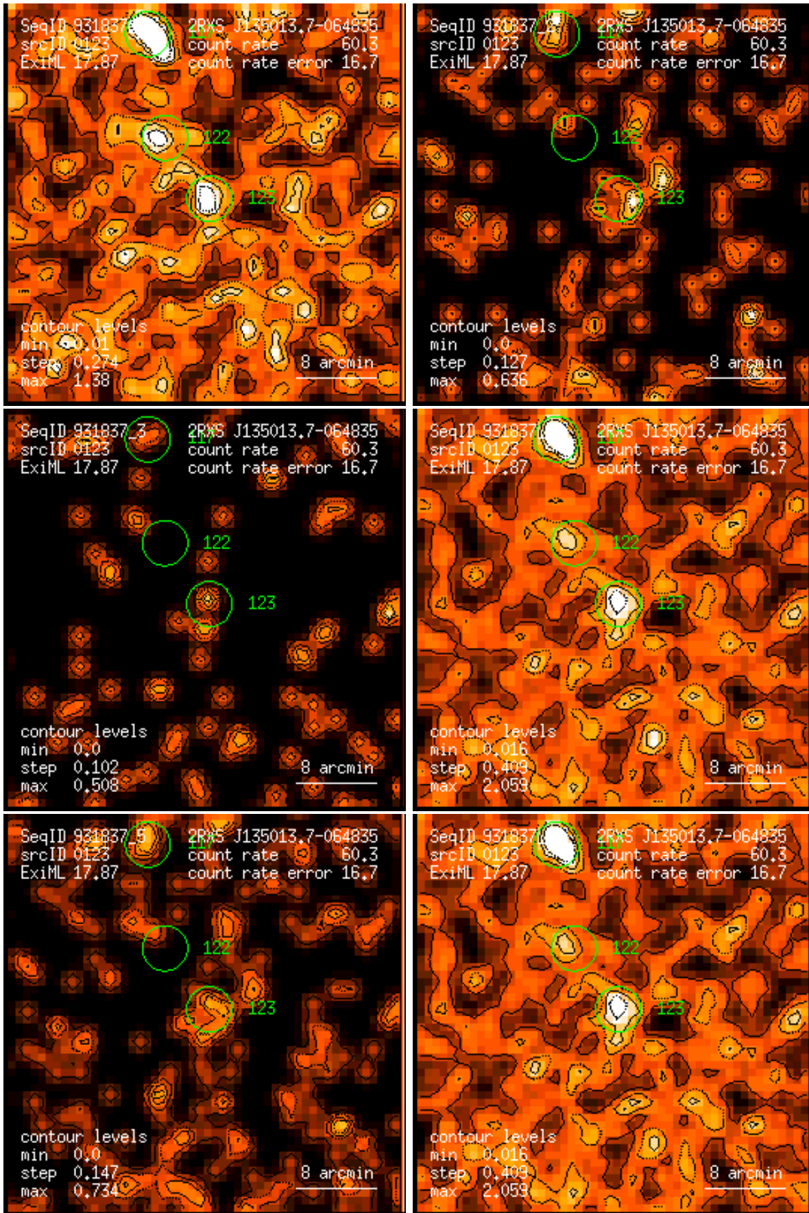
Figure 123: RASS 931837: detection 0123: band rate images, Gaussian filter: (1) PSPC channels 11 – 41, (2) 52 – 90, (3) 91 – 201, (4) 11 – 235, (5) 52 – 201, (6) 11 – 201. Broad band rates in counts/ks. Band rate contour levels in counts/ks/arcmin 2 .
