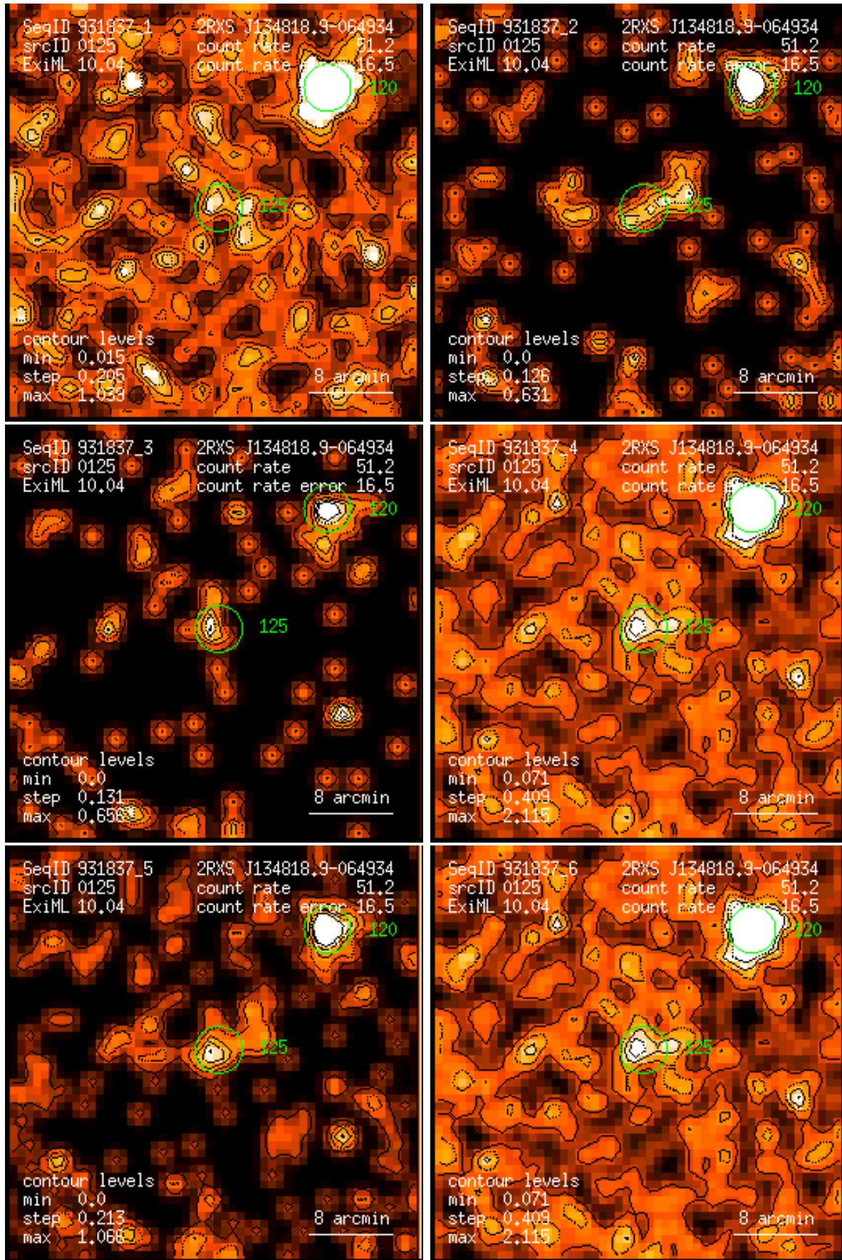
Figure 125: RASS 931837: detection 0125: band rate images, Gaussian filter: (1) PSPC channels 11 – 41, (2) 52 – 90, (3) 91 – 201, (4) 11 – 235, (5) 52 – 201, (6) 11 – 201. Broad band rates in counts/ks. Band rate contour levels in counts/ks/arcmin 2 .
