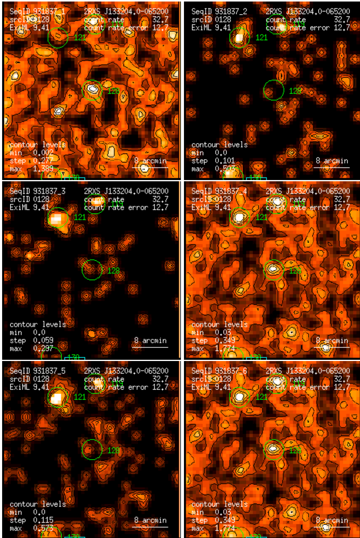
Figure 128: RASS 931837: detection 0128: band rate images, Gaussian filter: (1) PSPC channels 11 – 41, (2) 52 – 90, (3) 91 – 201, (4) 11 – 235, (5) 52 – 201, (6) 11 – 201. Broad band rates in counts/ks. Band rate contour levels in counts/ks/arcmin 2 .
