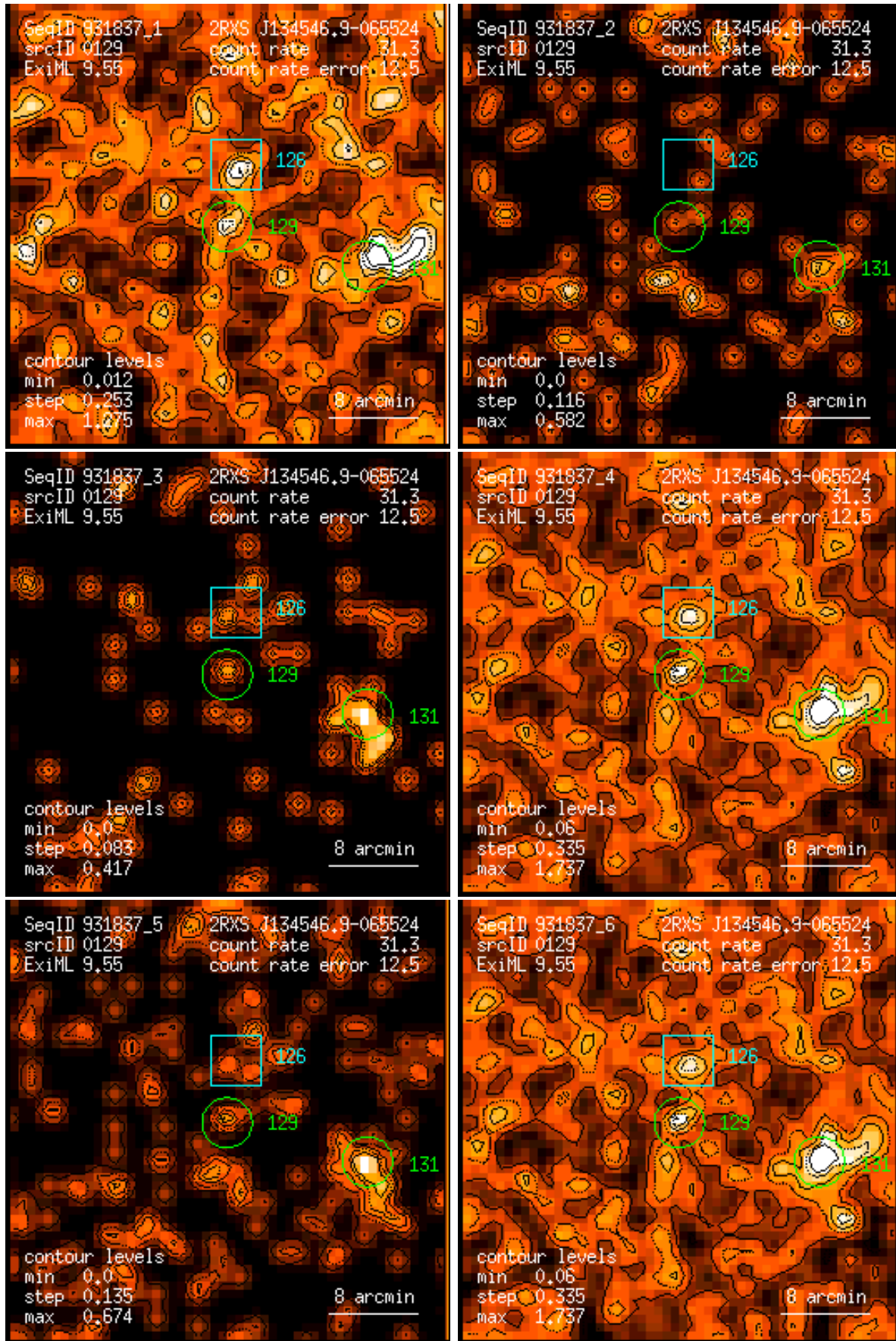
Figure 129: RASS 931837: detection 0129: band rate images, Gaussian filter: (1) PSPC channels 11 – 41, (2) 52 – 90, (3) 91 – 201, (4) 11 – 235, (5) 52 – 201, (6) 11 – 201. Broad band rates in counts/ks. Band rate contour levels in counts/ks/arcmin 2 .
