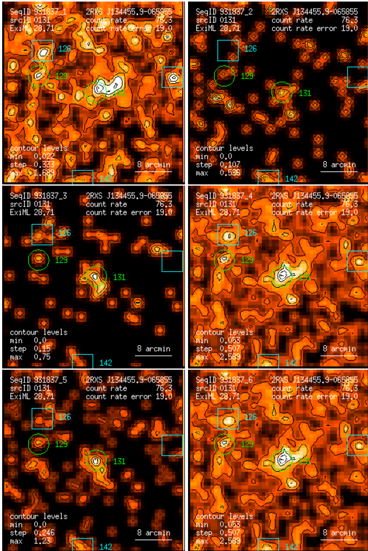
Figure 131: RASS 931837: detection 0131: band rate images, Gaussian filter: (1) PSPC channels 11 – 41, (2) 52 – 90, (3) 91 – 201, (4) 11 – 235, (5) 52 – 201, (6) 11 – 201. Broad band rates in counts/ks. Band rate contour levels in counts/ks/arcmin 2 .
