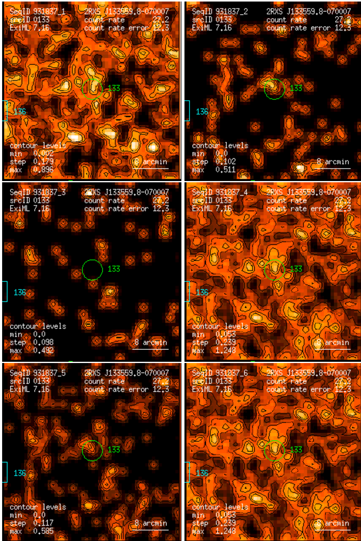
Figure 133: RASS 931837: detection 0133: band rate images, Gaussian filter: (1) PSPC channels 11 – 41, (2) 52 – 90, (3) 91 – 201, (4) 11 – 235, (5) 52 – 201, (6) 11 – 201. Broad band rates in counts/ks. Band rate contour levels in counts/ks/arcmin 2 .
