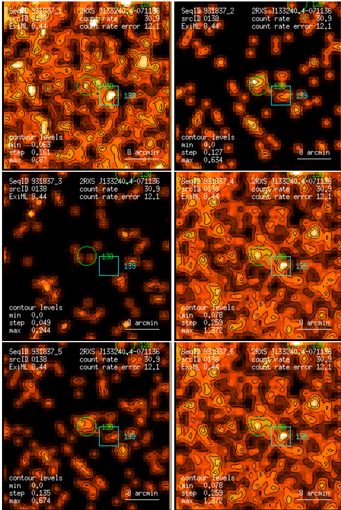
Figure 138: RASS 931837: detection 0138: band rate images, Gaussian filter: (1) PSPC channels 11 – 41, (2) 52 – 90, (3) 91 – 201, (4) 11 – 235, (5) 52 – 201, (6) 11 – 201. Broad band rates in counts/ks. Band rate contour levels in counts/ks/arcmin 2 .
