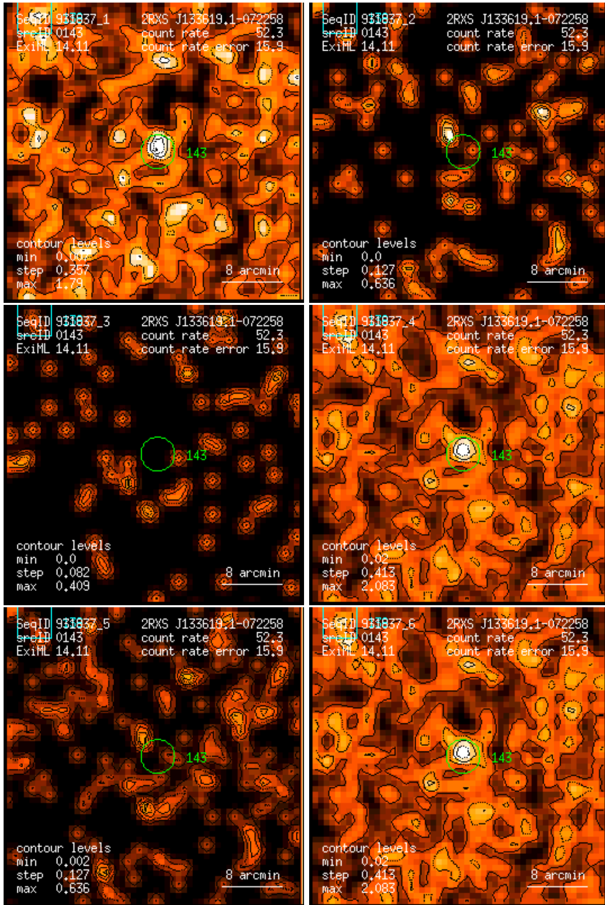
Figure 143: RASS 931837: detection 0143: band rate images, Gaussian filter: (1) PSPC channels 11 – 41, (2) 52 – 90, (3) 91 – 201, (4) 11 – 235, (5) 52 – 201, (6) 11 – 201. Broad band rates in counts/ks. Band rate contour levels in counts/ks/arcmin 2 .
