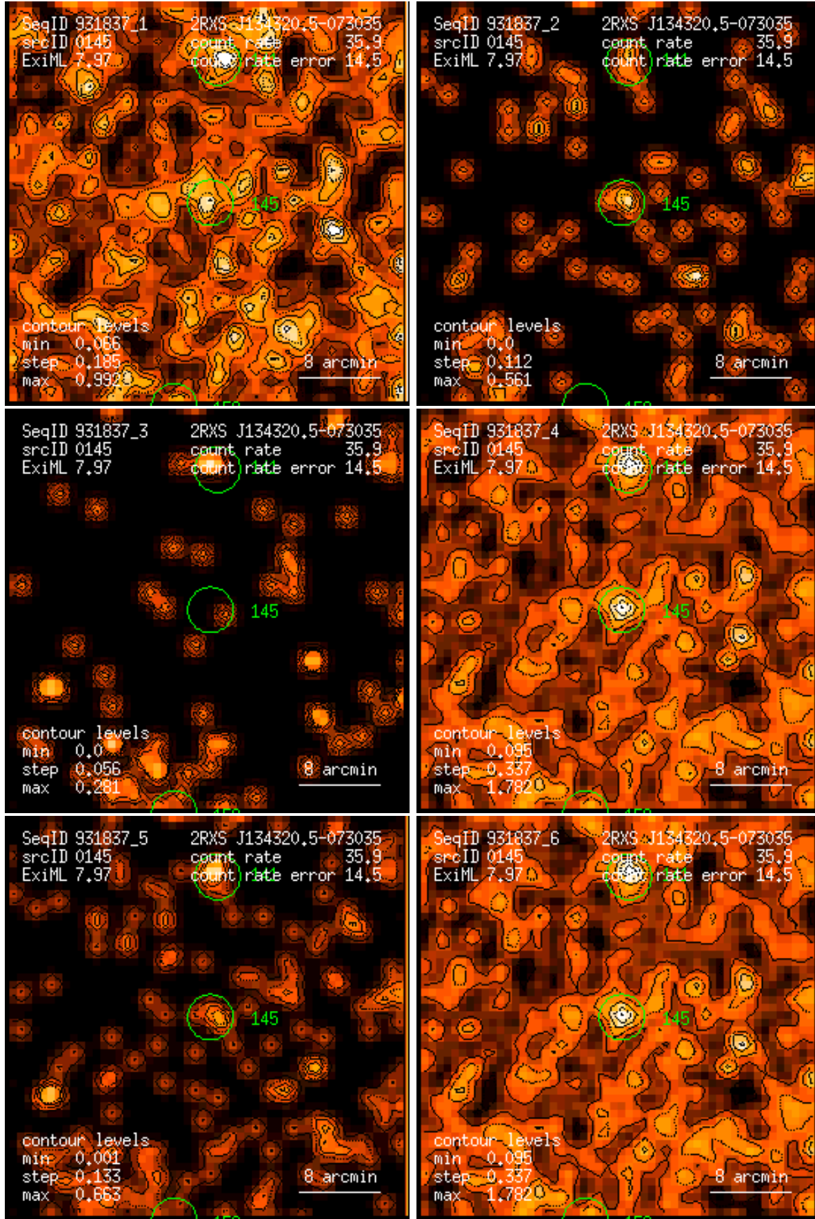
Figure 145: RASS 931837: detection 0145: band rate images, Gaussian filter: (1) PSPC channels 11 – 41, (2) 52 – 90, (3) 91 – 201, (4) 11 – 235, (5) 52 – 201, (6) 11 – 201. Broad band rates in counts/ks. Band rate contour levels in counts/ks/arcmin 2 .
