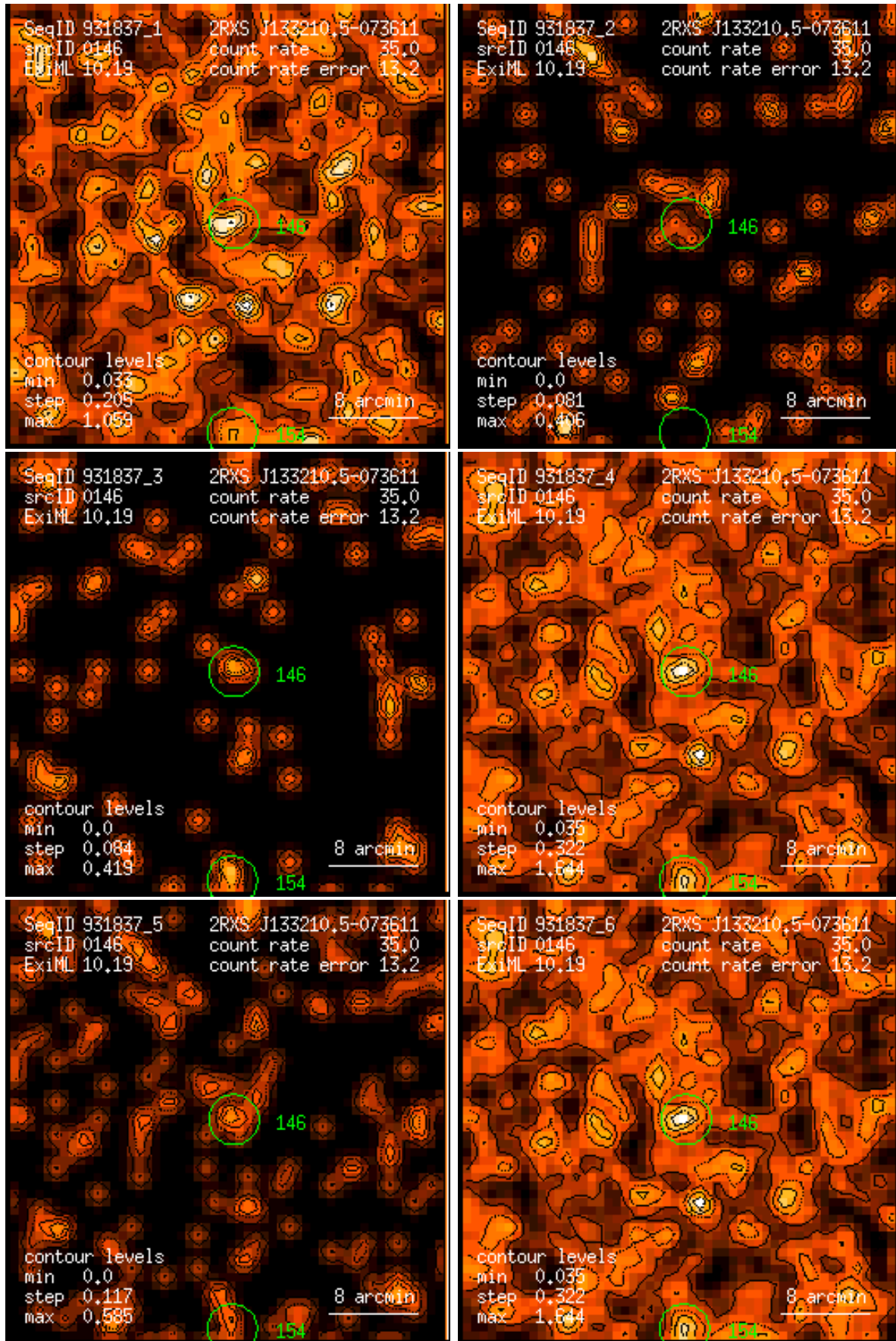
Figure 146: RASS 931837: detection 0146: band rate images, Gaussian filter: (1) PSPC channels 11 – 41, (2) 52 – 90, (3) 91 – 201, (4) 11 – 235, (5) 52 – 201, (6) 11 – 201. Broad band rates in counts/ks. Band rate contour levels in counts/ks/arcmin 2 .
