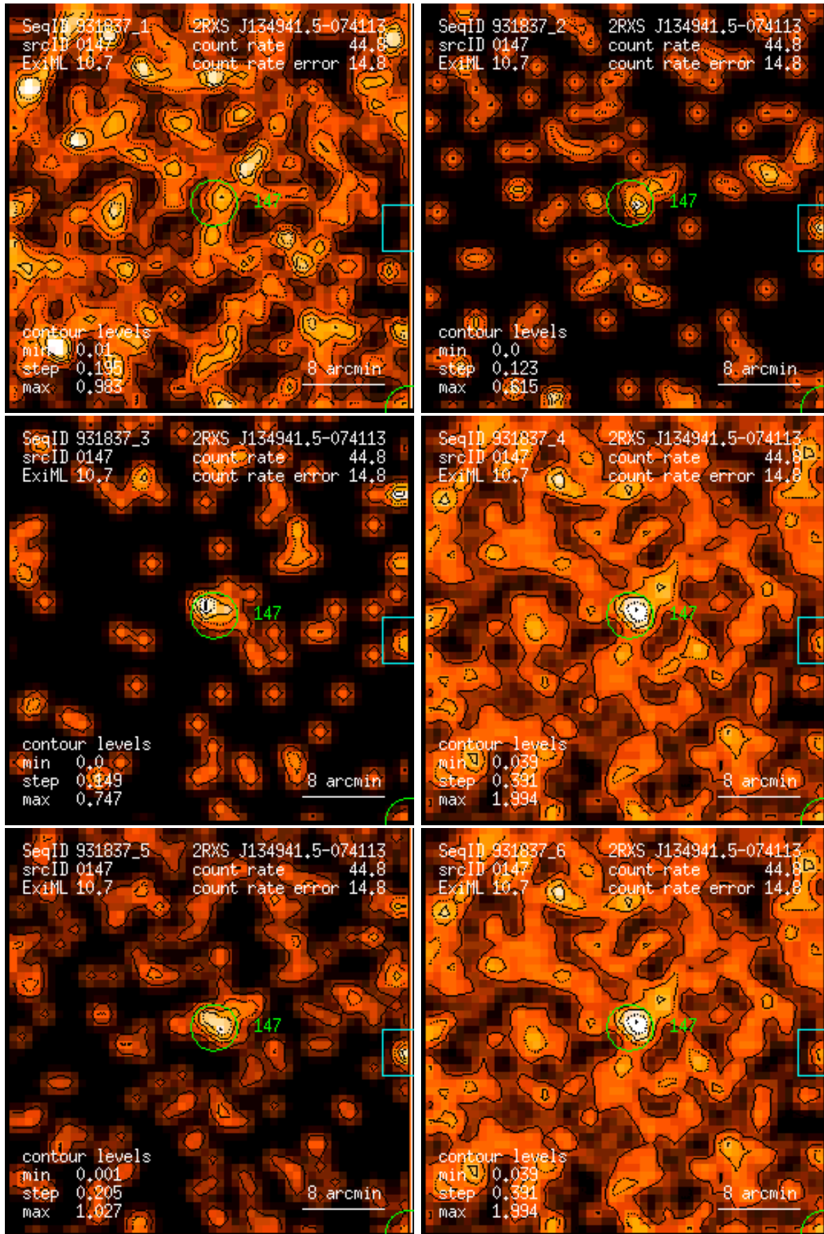
Figure 147: RASS 931837: detection 0147: band rate images, Gaussian filter: (1) PSPC channels 11 – 41, (2) 52 – 90, (3) 91 – 201, (4) 11 – 235, (5) 52 – 201, (6) 11 – 201. Broad band rates in counts/ks. Band rate contour levels in counts/ks/arcmin 2 .
