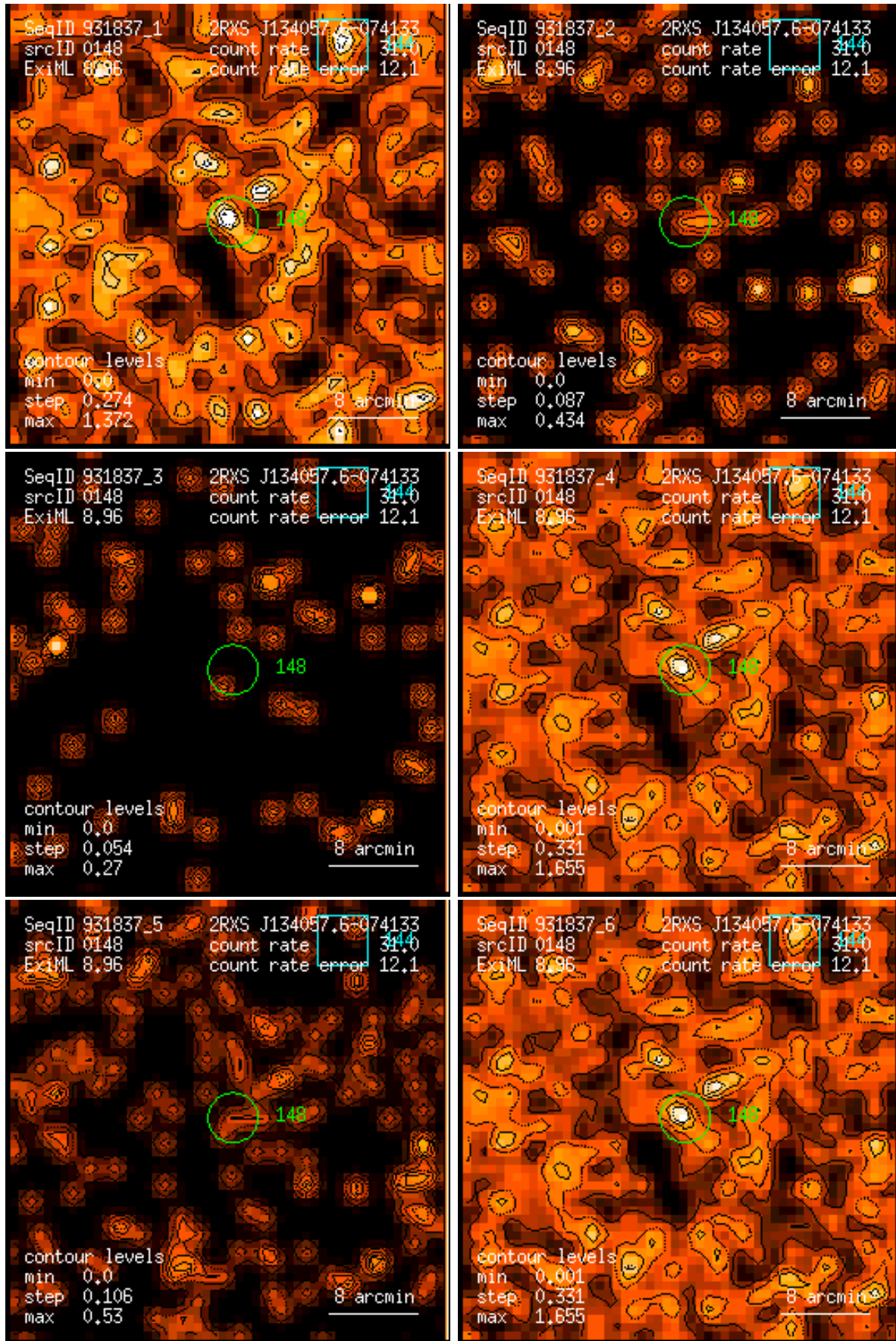
Figure 148: RASS 931837: detection 0148: band rate images, Gaussian filter: (1) PSPC channels 11 – 41, (2) 52 – 90, (3) 91 – 201, (4) 11 – 235, (5) 52 – 201, (6) 11 – 201. Broad band rates in counts/ks. Band rate contour levels in counts/ks/arcmin 2 .
