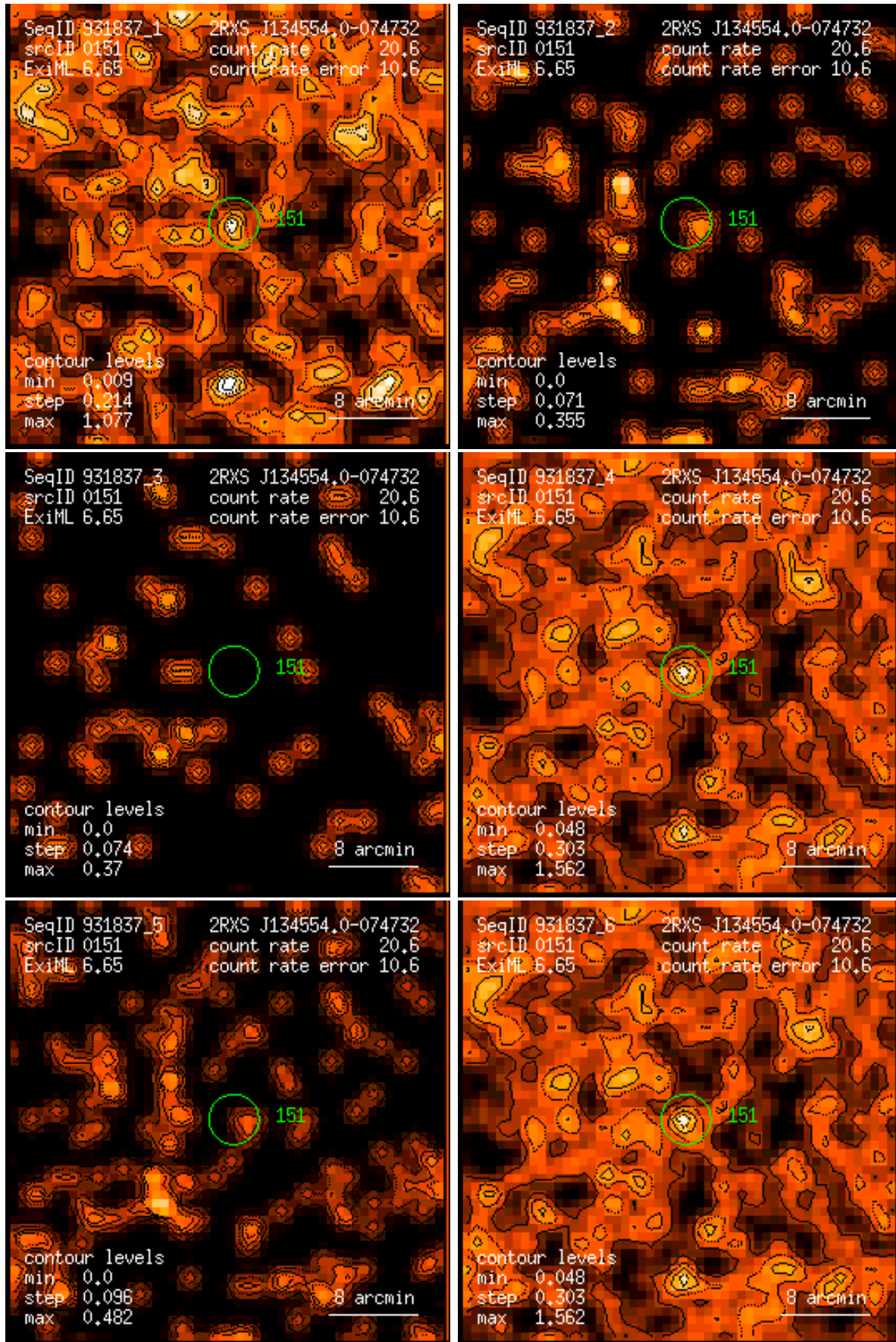
Figure 151: RASS 931837: detection 0151: band rate images, Gaussian filter: (1) PSPC channels 11 – 41, (2) 52 – 90, (3) 91 – 201, (4) 11 – 235, (5) 52 – 201, (6) 11 – 201. Broad band rates in counts/ks. Band rate contour levels in counts/ks/arcmin 2 .
