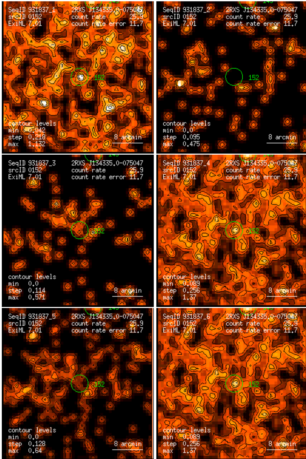
Figure 152: RASS 931837: detection 0152: band rate images, Gaussian filter: (1) PSPC channels 11 – 41, (2) 52 – 90, (3) 91 – 201, (4) 11 – 235, (5) 52 – 201, (6) 11 – 201. Broad band rates in counts/ks. Band rate contour levels in counts/ks/arcmin 2 .
