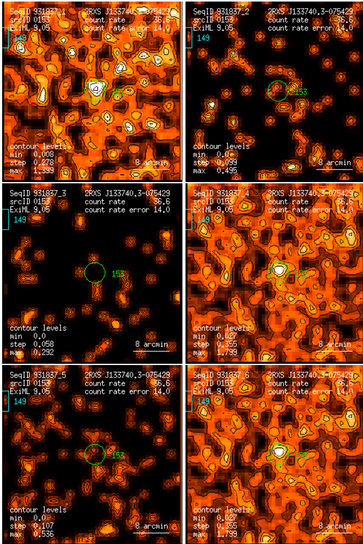
Figure 153: RASS 931837: detection 0153: band rate images, Gaussian filter: (1) PSPC channels 11 – 41, (2) 52 – 90, (3) 91 – 201, (4) 11 – 235, (5) 52 – 201, (6) 11 – 201. Broad band rates in counts/ks. Band rate contour levels in counts/ks/arcmin 2 .
