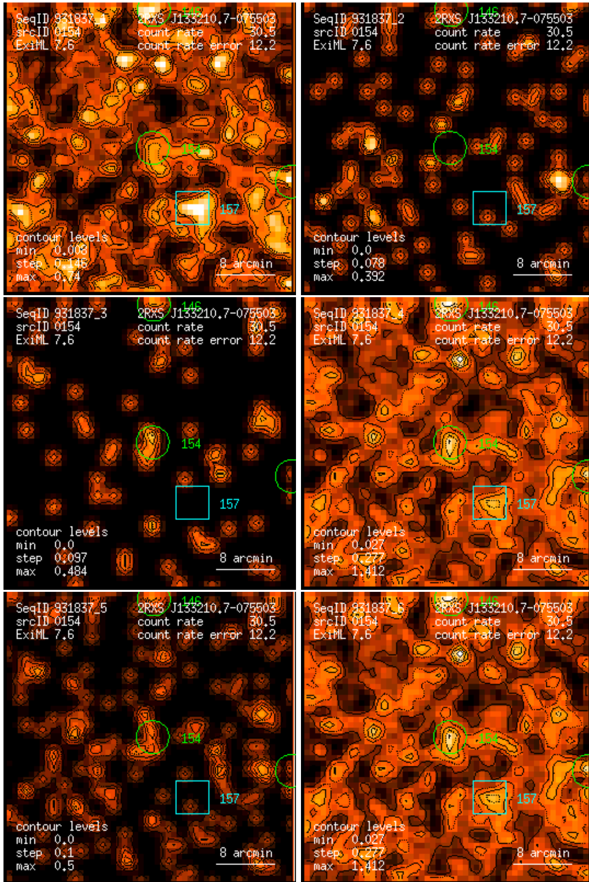
Figure 154: RASS 931837: detection 0154: band rate images, Gaussian filter: (1) PSPC channels 11 – 41, (2) 52 – 90, (3) 91 – 201, (4) 11 – 235, (5) 52 – 201, (6) 11 – 201. Broad band rates in counts/ks. Band rate contour levels in counts/ks/arcmin 2 .
