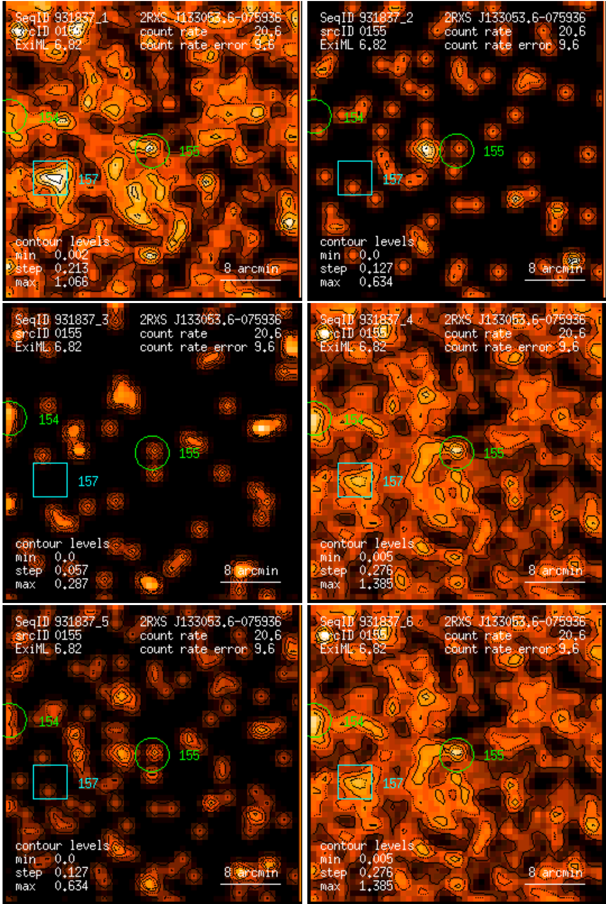
Figure 155: RASS 931837: detection 0155: band rate images, Gaussian filter: (1) PSPC channels 11 – 41, (2) 52 – 90, (3) 91 – 201, (4) 11 – 235, (5) 52 – 201, (6) 11 – 201. Broad band rates in counts/ks. Band rate contour levels in counts/ks/arcmin 2 .
