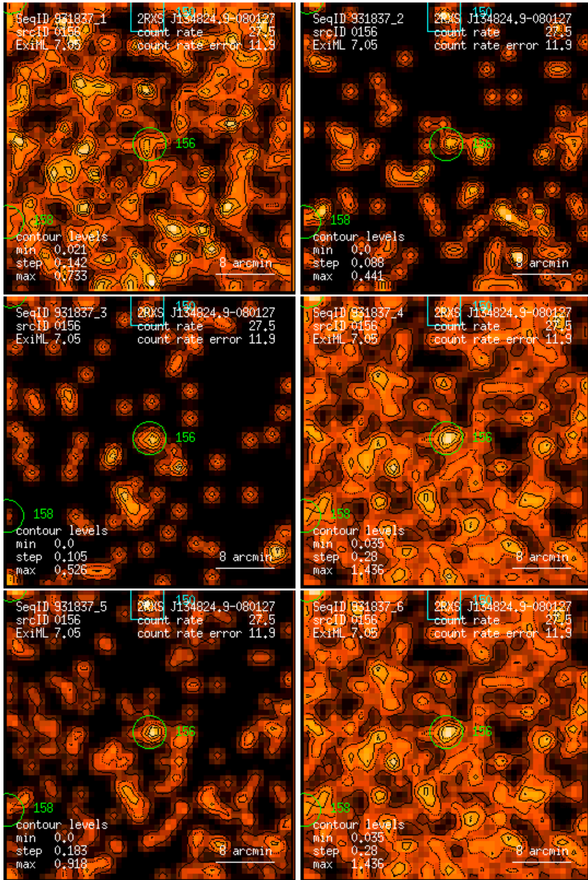
Figure 156: RASS 931837: detection 0156: band rate images, Gaussian filter: (1) PSPC channels 11 – 41, (2) 52 – 90, (3) 91 – 201, (4) 11 – 235, (5) 52 – 201, (6) 11 – 201. Broad band rates in counts/ks. Band rate contour levels in counts/ks/arcmin 2 .
