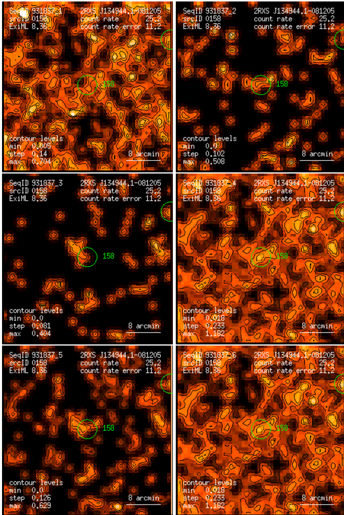
Figure 158: RASS 931837: detection 0158: band rate images, Gaussian filter: (1) PSPC channels 11 – 41, (2) 52 – 90, (3) 91 – 201, (4) 11 – 235, (5) 52 – 201, (6) 11 – 201. Broad band rates in counts/ks. Band rate contour levels in counts/ks/arcmin 2 .
