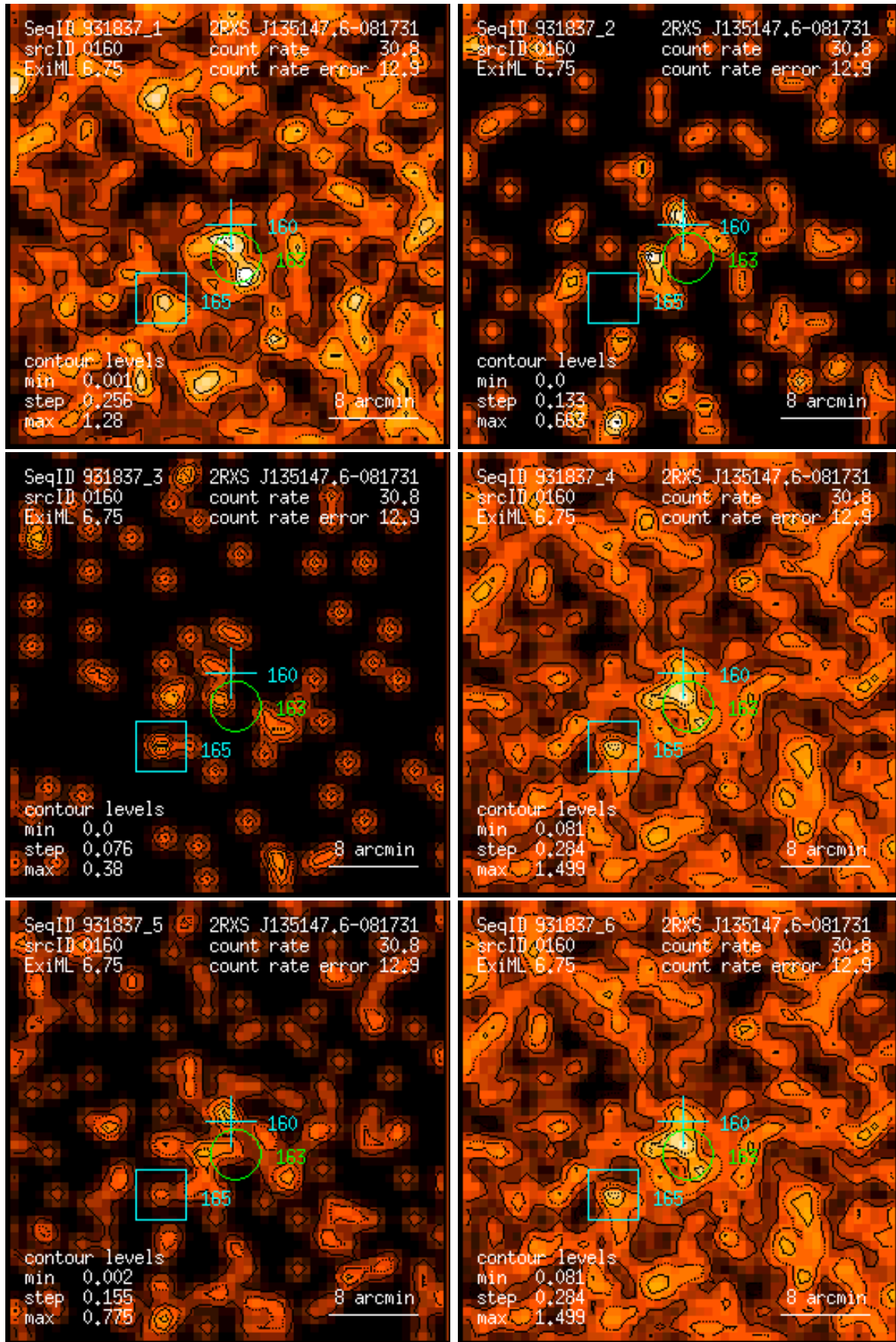
Figure 160: RASS 931837: detection 0160: band rate images, Gaussian filter: (1) PSPC channels 11 – 41, (2) 52 – 90, (3) 91 – 201, (4) 11 – 235, (5) 52 – 201, (6) 11 – 201. Broad band rates in counts/ks. Band rate contour levels in counts/ks/arcmin 2 .
