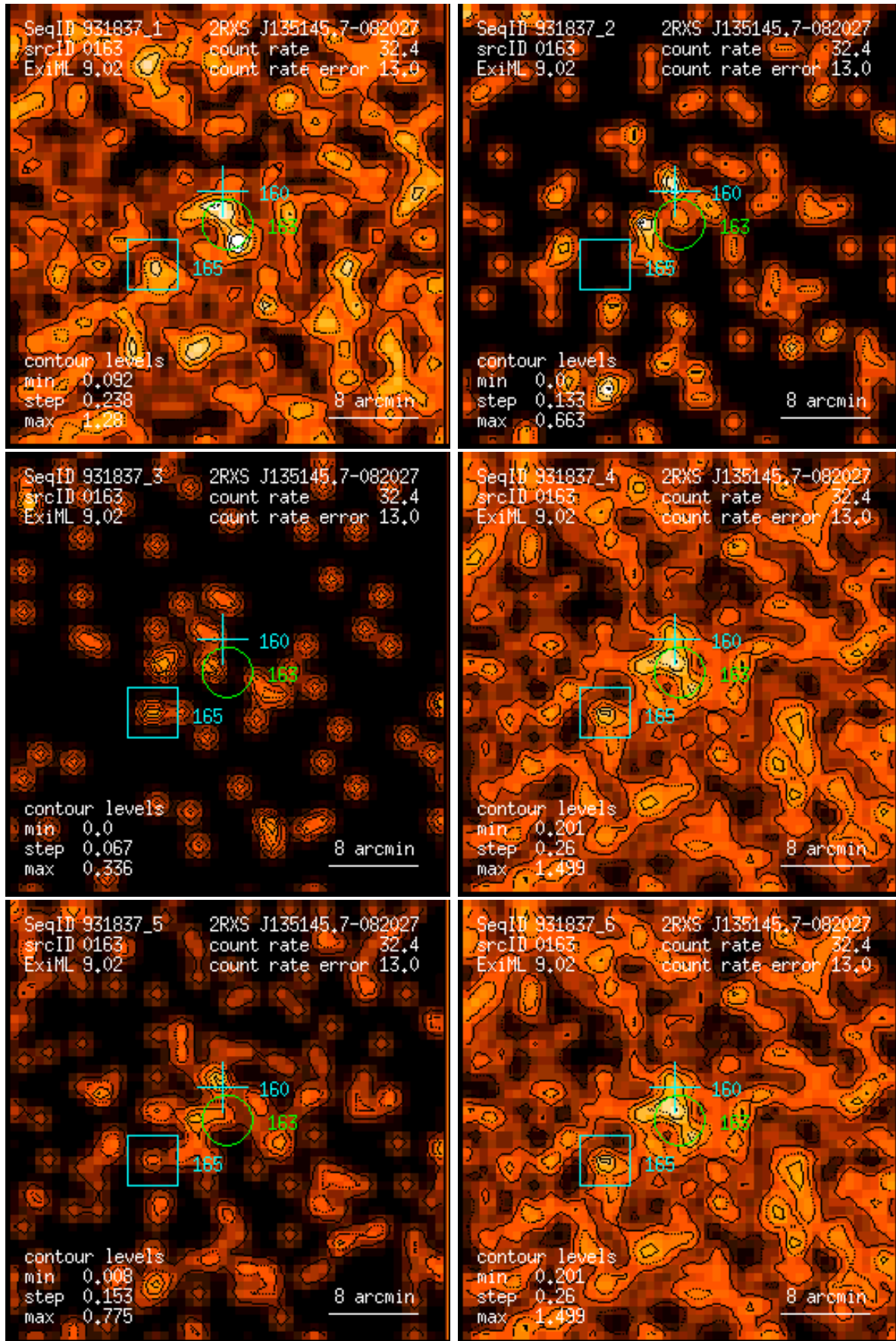
Figure 163: RASS 931837: detection 0163: band rate images, Gaussian filter: (1) PSPC channels 11 – 41, (2) 52 – 90, (3) 91 – 201, (4) 11 – 235, (5) 52 – 201, (6) 11 – 201. Broad band rates in counts/ks. Band rate contour levels in counts/ks/arcmin 2 .
