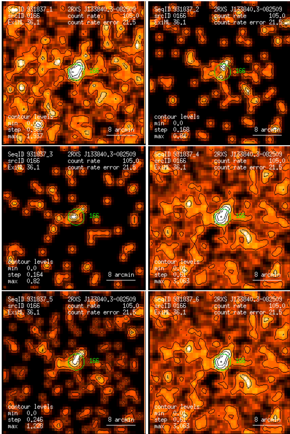
Figure 166: RASS 931837: detection 0166: band rate images, Gaussian filter: (1) PSPC channels 11 – 41, (2) 52 – 90, (3) 91 – 201, (4) 11 – 235, (5) 52 – 201, (6) 11 – 201. Broad band rates in counts/ks. Band rate contour levels in counts/ks/arcmin 2 .
